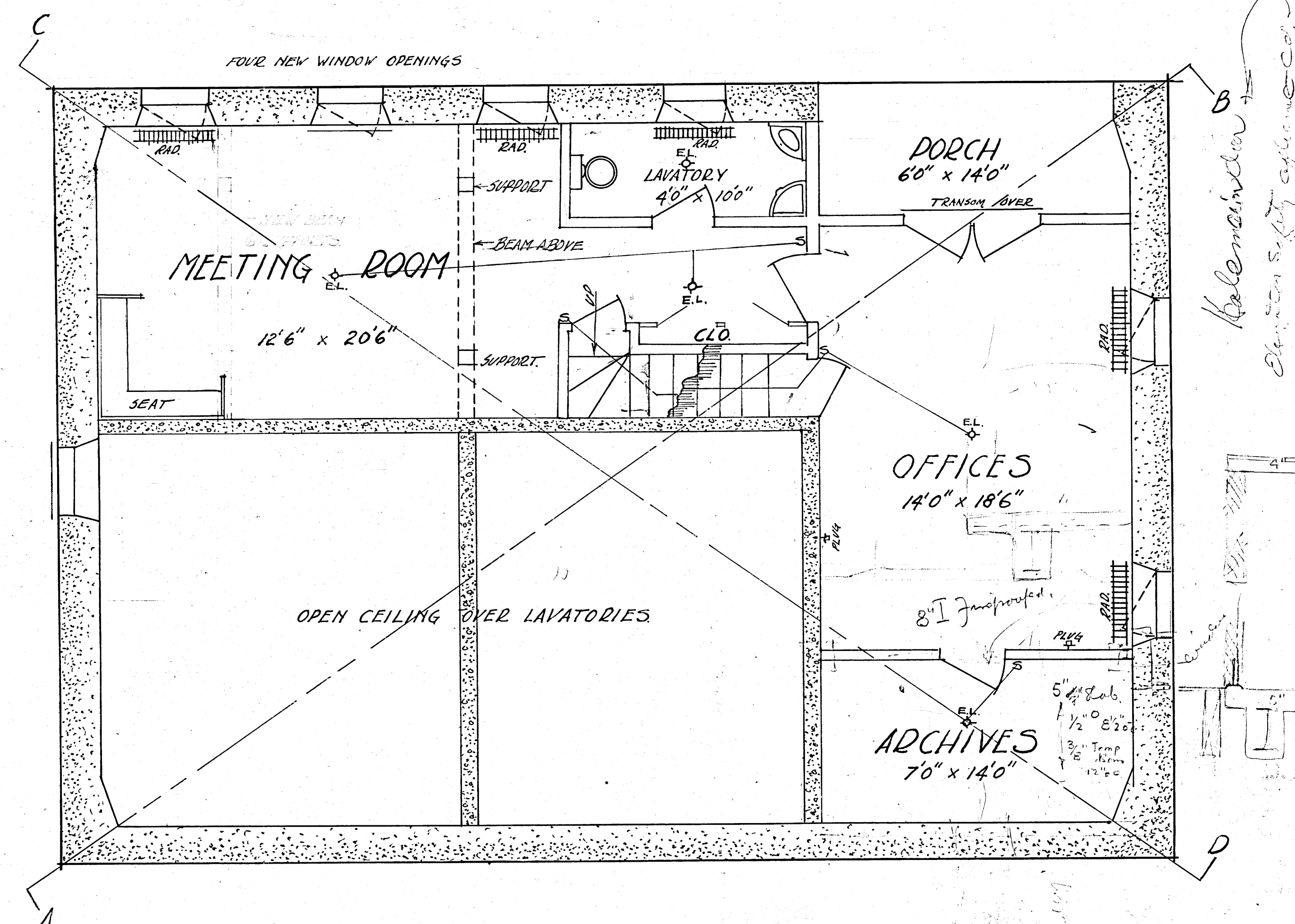
SECOND FLOOR
