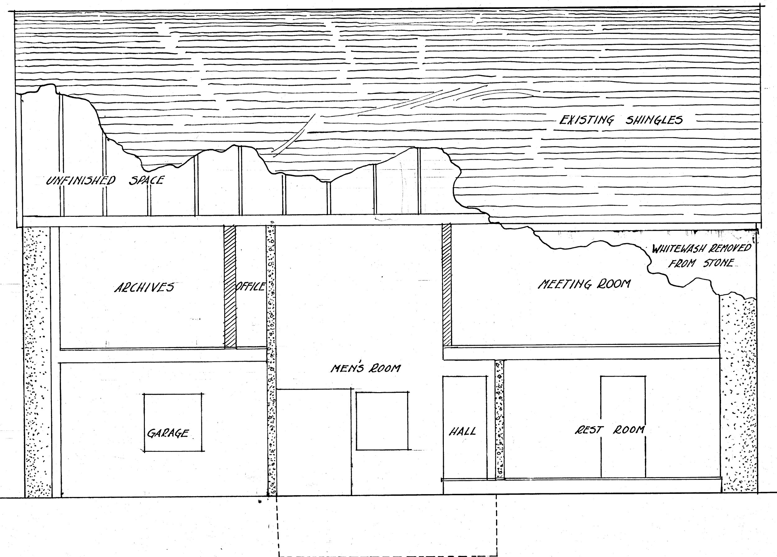
SECTION FROM EAST ON C-D.
