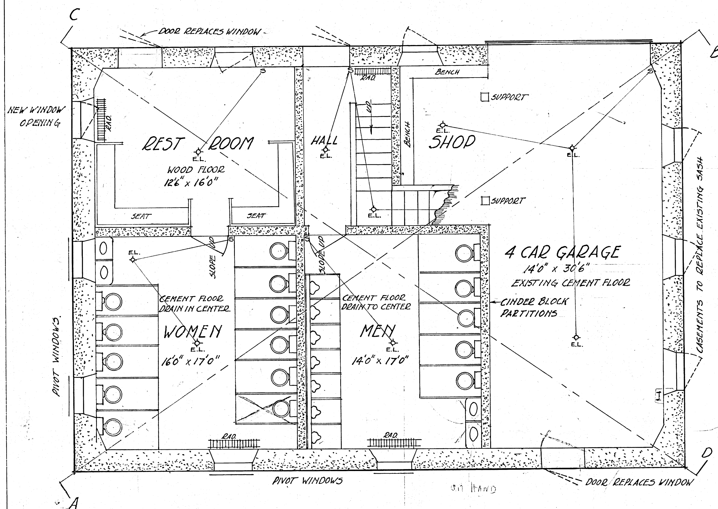
FIRST FLOOR
