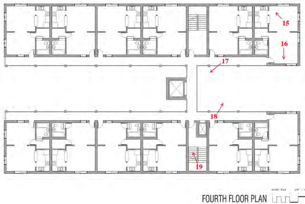
Figure 6. Floor Plan/Photo Key—Fourth Floor
