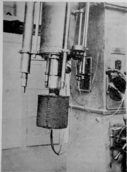
FIG. 1.—Selenium Cell in Ice-Pack Attached to 12-Inch Refractor
