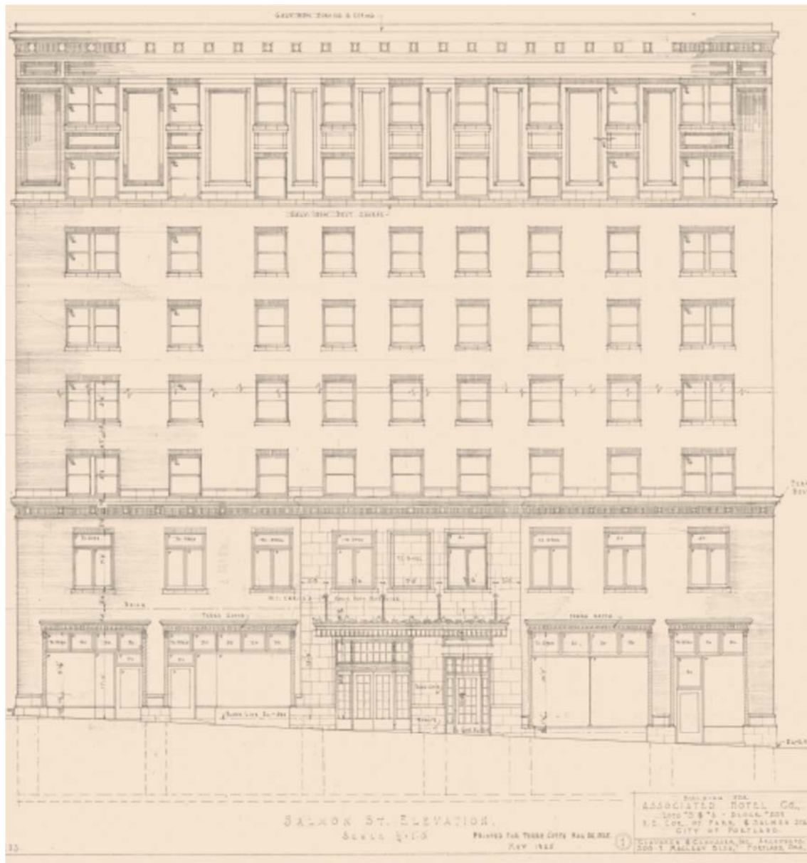
Figure 4: South Elevation, Heathman Hotel, Clausen and Clausen drawing, May 1925
