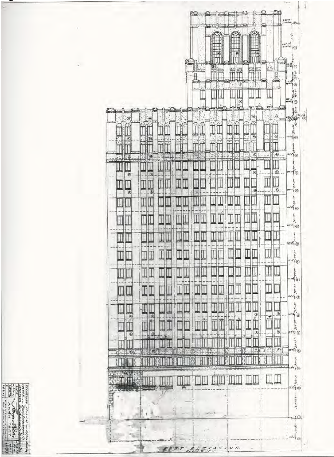
Figure 19: East Elevation.
