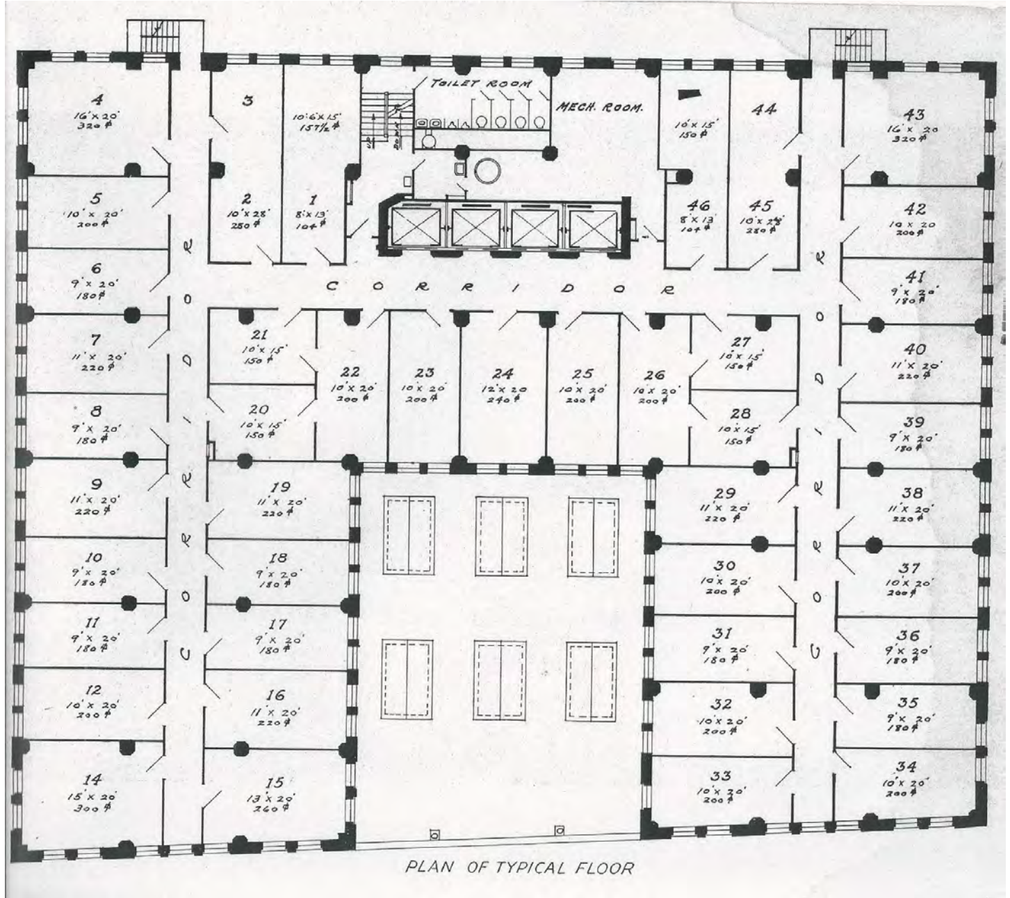
Figure 20. Floor plan
