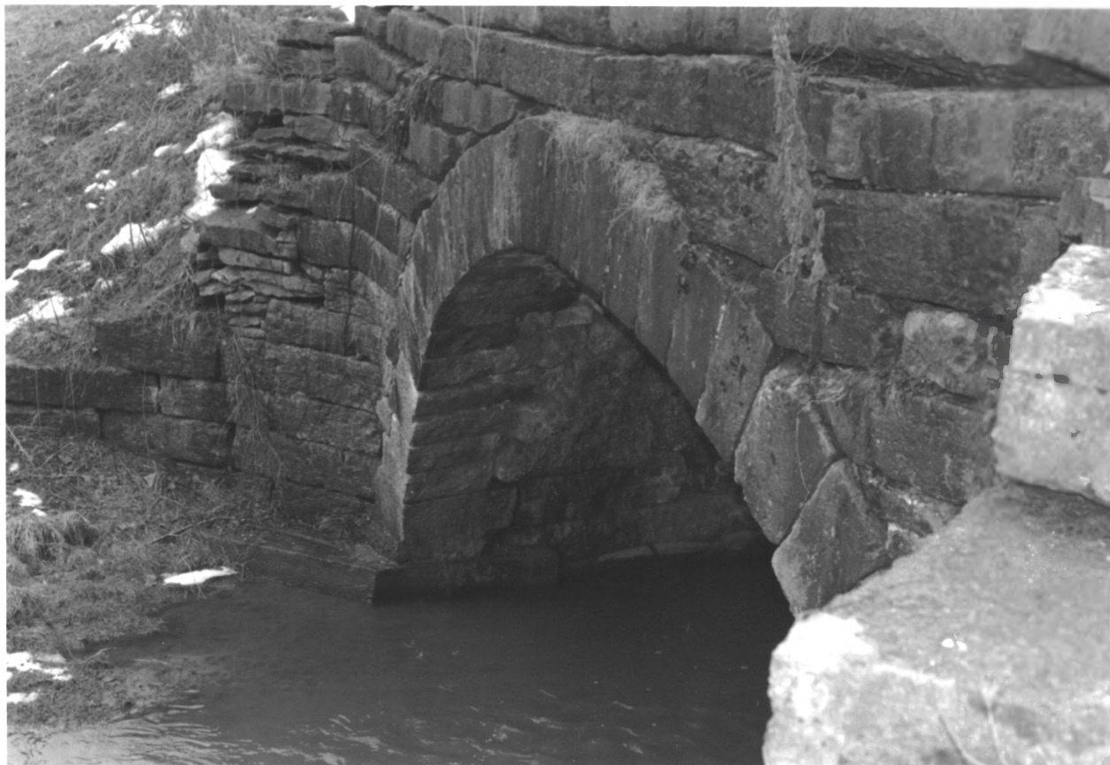
WABASH AND ERIE CANAL CULVERT CARROLL CO., INDIANA 12A
