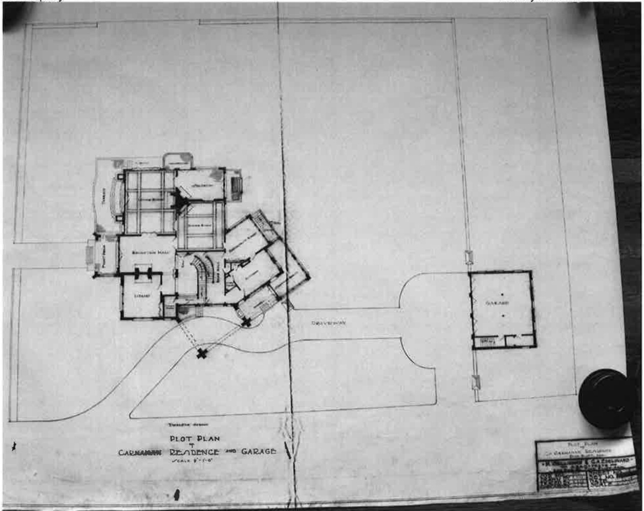
"Plot Plan of Carnahan Residence and Garage, Pine Bluff, ARK., M. Selligman & G. A. Edelsvard, Architects, Pine Bluff, ARK." November 26, 1919.
