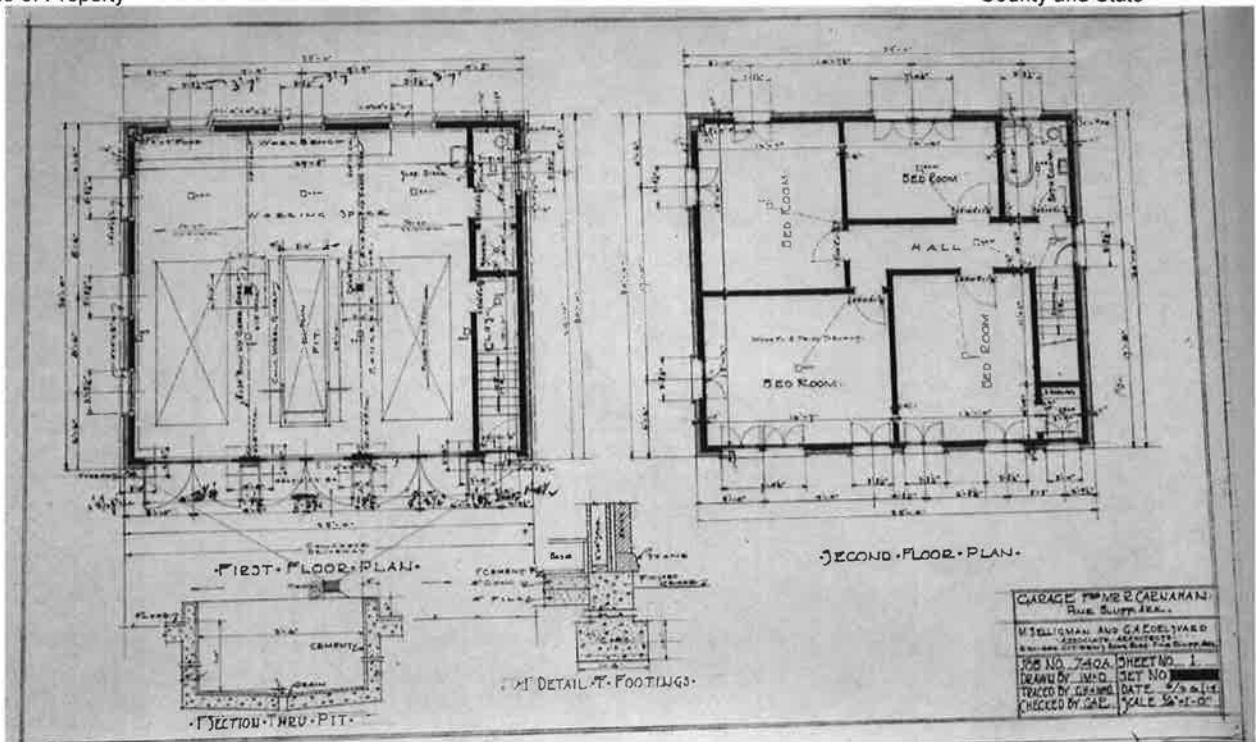
Plan Drawings, First and Second Floor Plans. "Garage for Mr. R. Carnahan, Pine Bluff, ARK., M. Selligman And G. A. Edelsvard, Associate Architects, 601-602 Citizens Bank Bldg. Pine Bluff, ARK." June 26, 1919.
