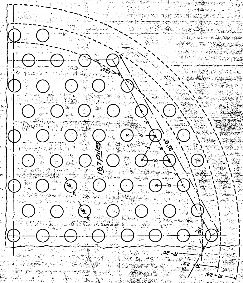
Part Plan, Pile Foundation Fig. 2
