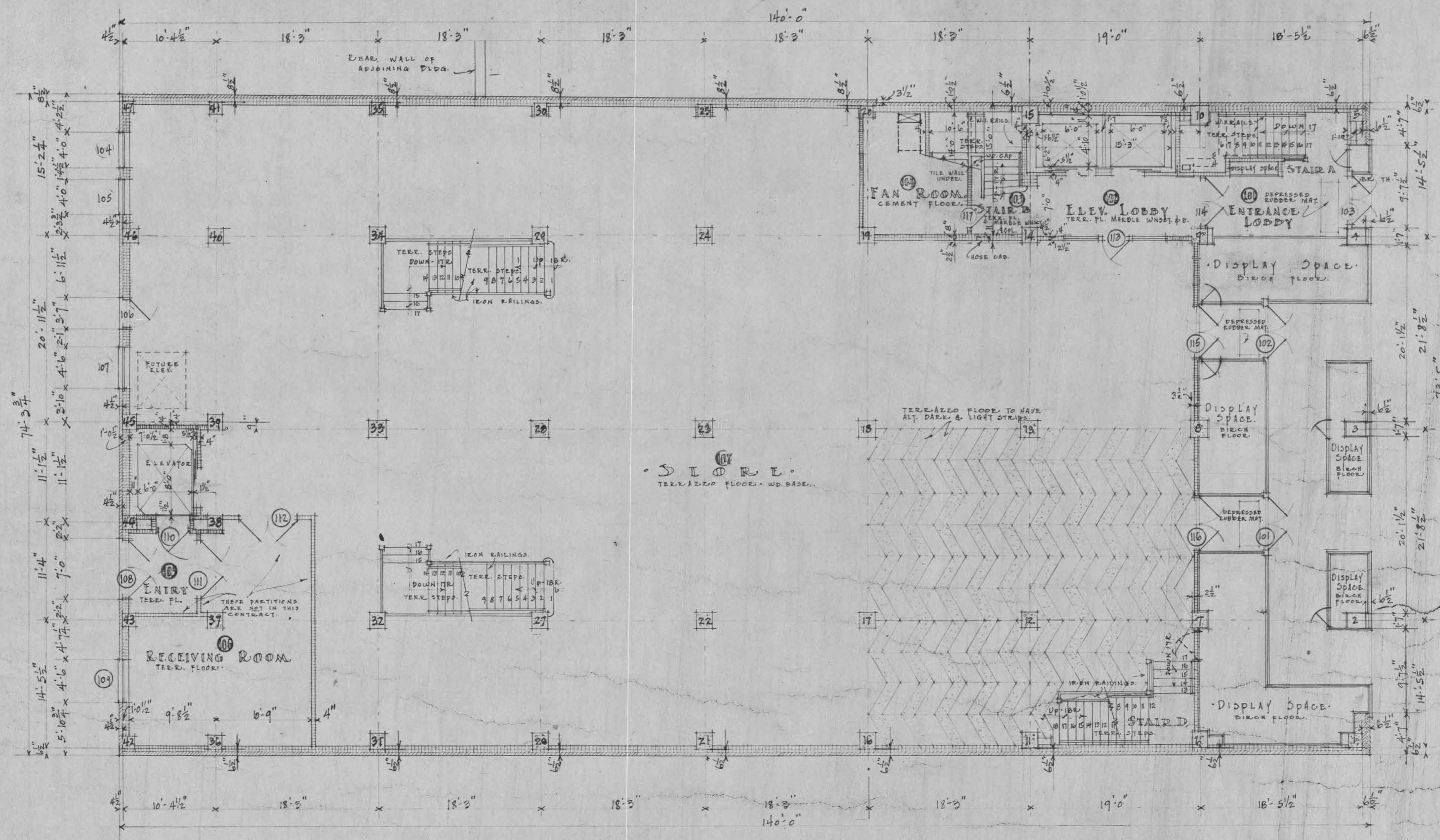
FIRST FLOOR PLAN SCALE 1/8"=1'-0"
