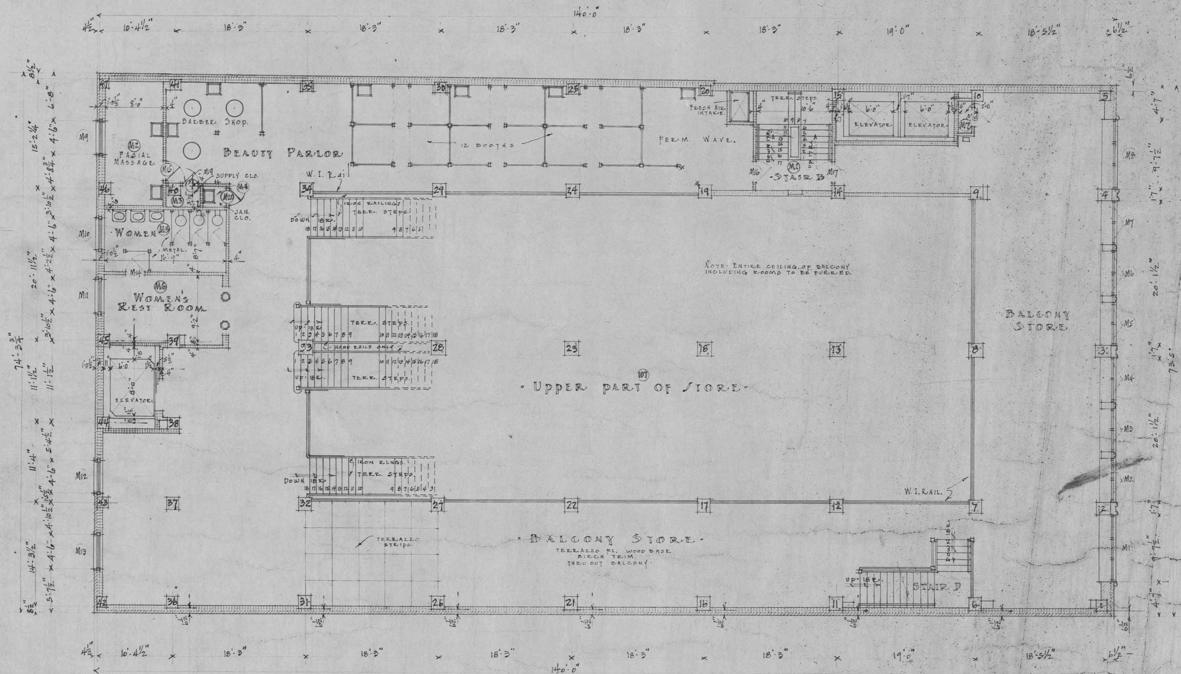
BALCONY FLOOR PLAN SCALE 1/8"=1'-0"
