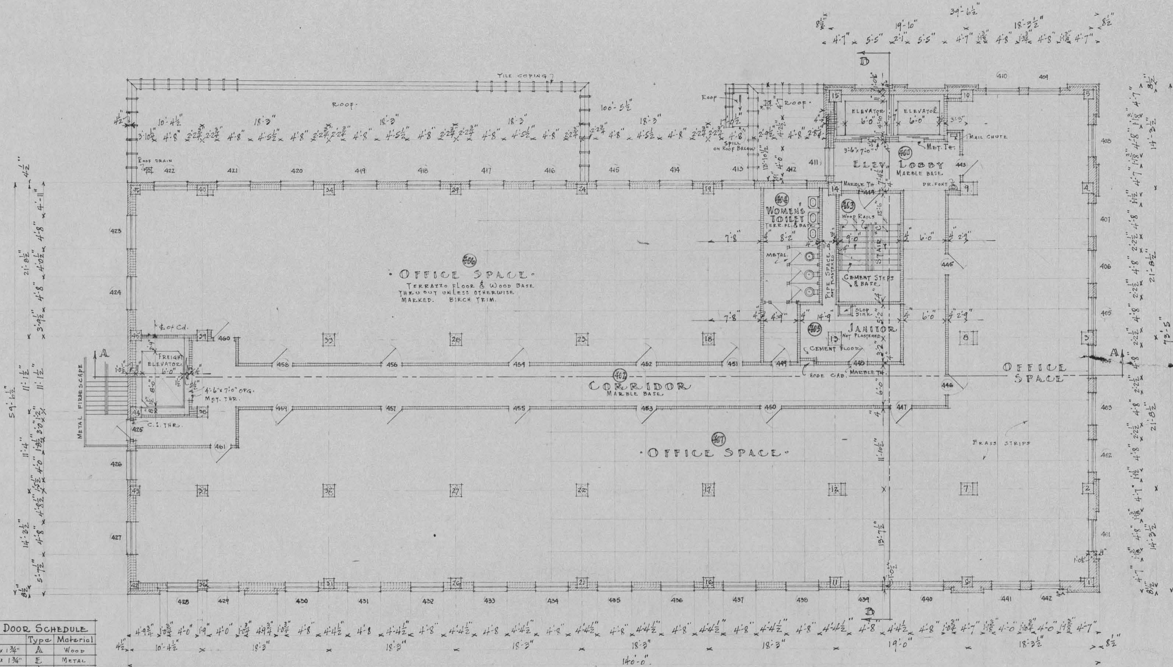
FOURTH FLOOR PLAN SCALE - 1/8" = 1'-0" 5TH, 6TH & 7TH FLOORS SIMILAR.
