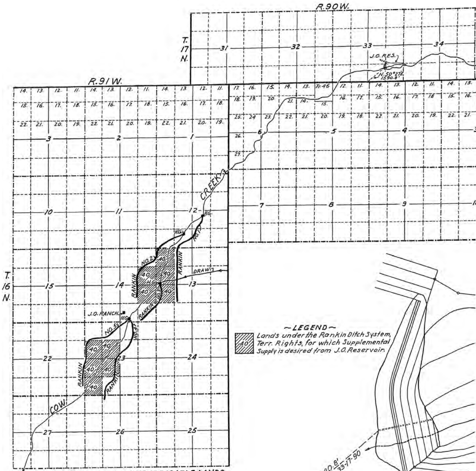
VICINITY MAP SHOWING IRRIGABLE LANDS SCALE 2"=1 MILE
