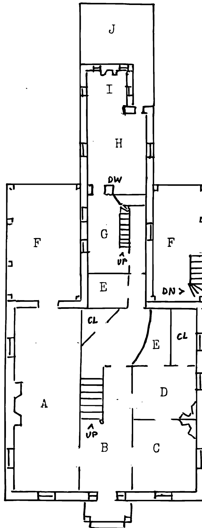
PLAN OF FIRST FLOOR. (Not to scale).
