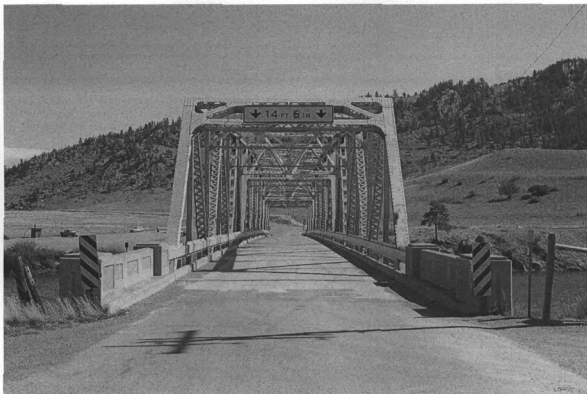
Photo 0005. Missouri River Bridge. West portal. View to the northeast.
