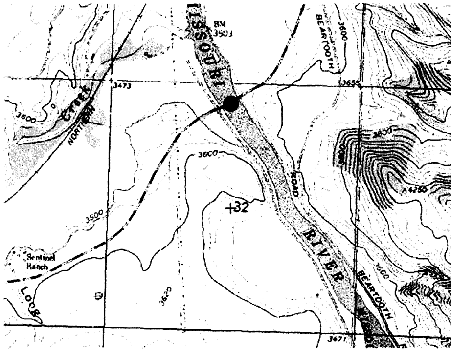
Location of Missouri River Bridge (T15N R3W S32 Wolf Creek 7.5' quadrangle map, 1979)
