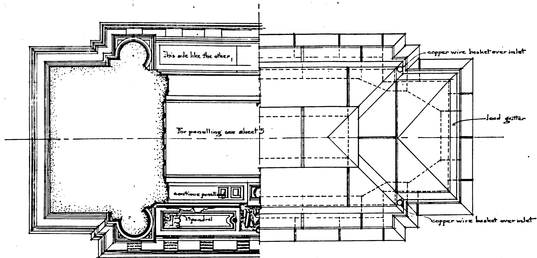
HALF PLAN OF ROOF
