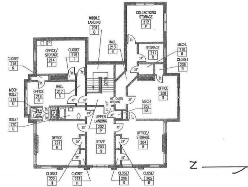
EXISTING CONDITIONS SECOND FLOOR PLAN 1/8" = 1'-0"
