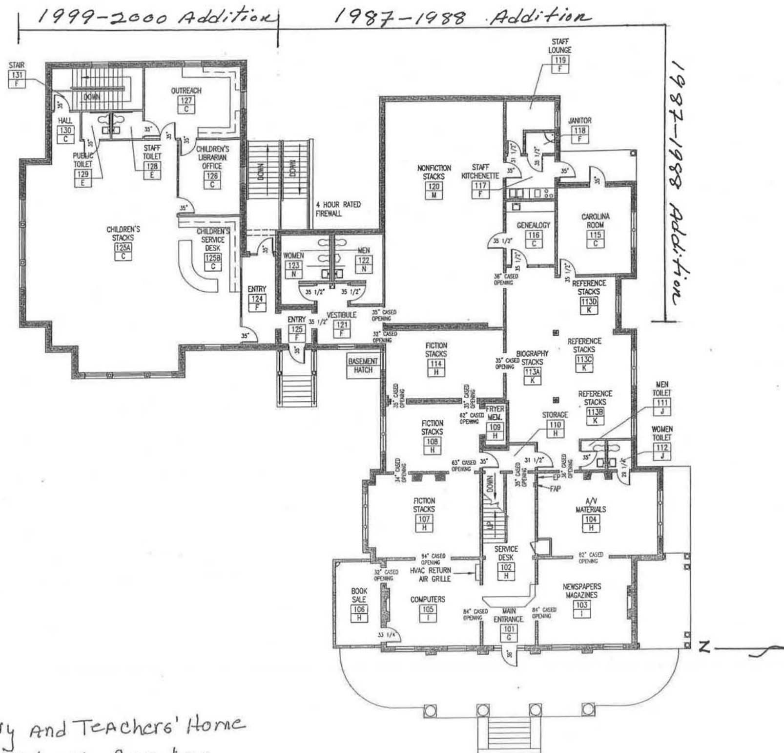
EXISTING CONDITIONS MAIN/FIRST FLOOR PLAN
