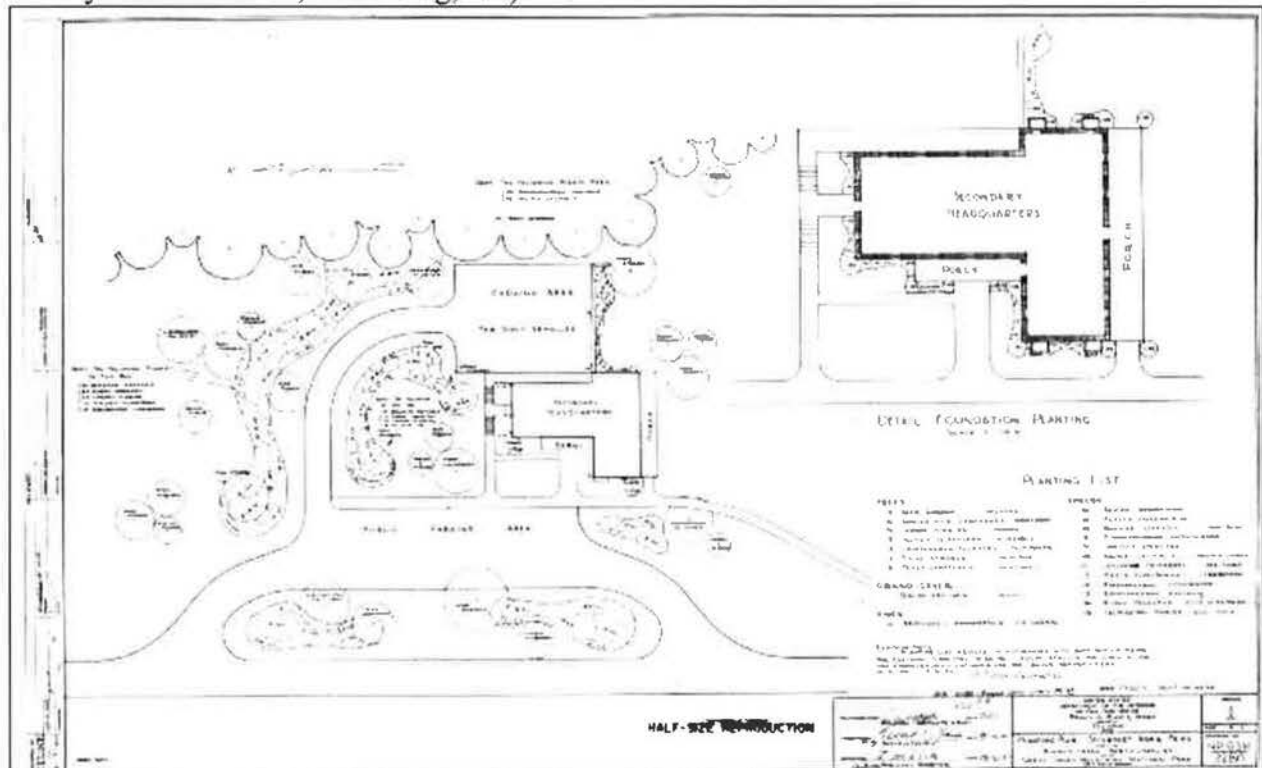
Figure 7. Planting Plan, Oconaluftee Ranger Station. Drawing NP-GSM 2280, 1940 (source: NPS Technical Information Center, Denver, CO).
