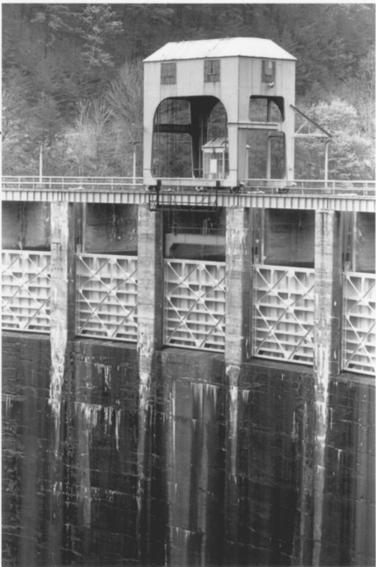
Calderwood Hydroelectric Station Calderwood vicinity, Blount & Monroe Cos, TN # 7089
