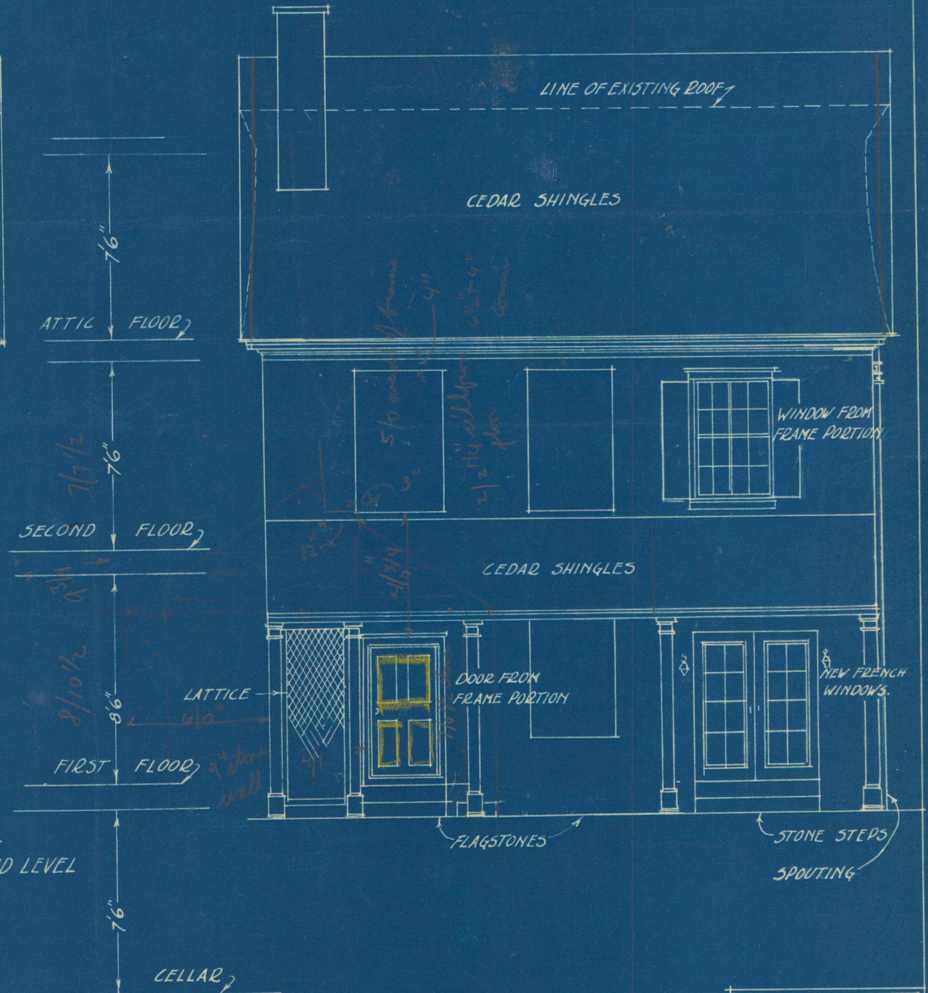
EAST ELEVATION
