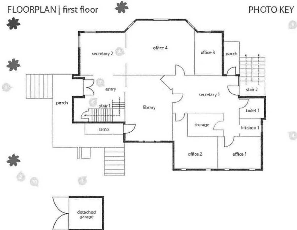
Figure 2 First Floor Plan. Courtesy of M-Group
