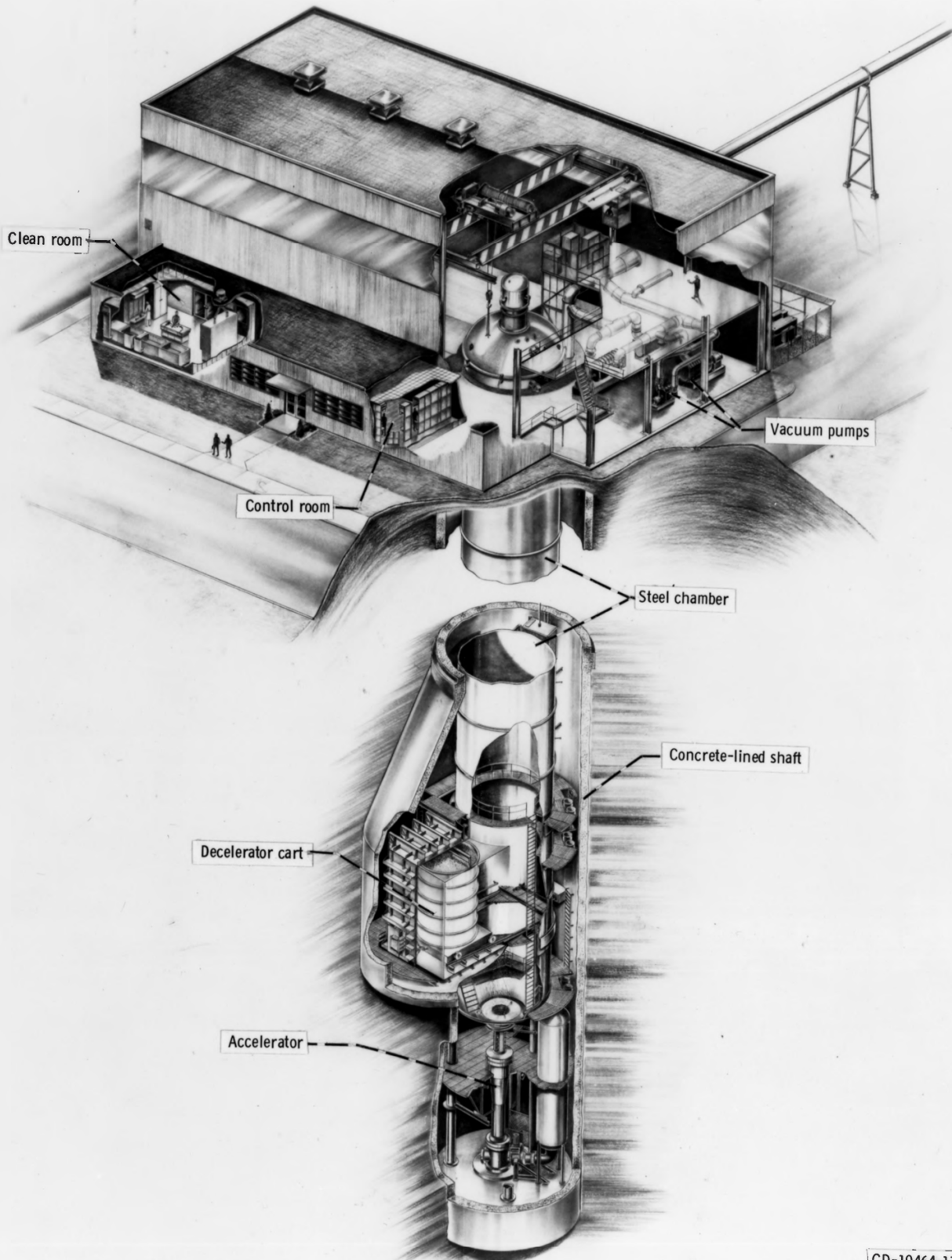
Figure 12. - Schematic diagram of 5- to 10-Second Zero-Gravity Facility.
