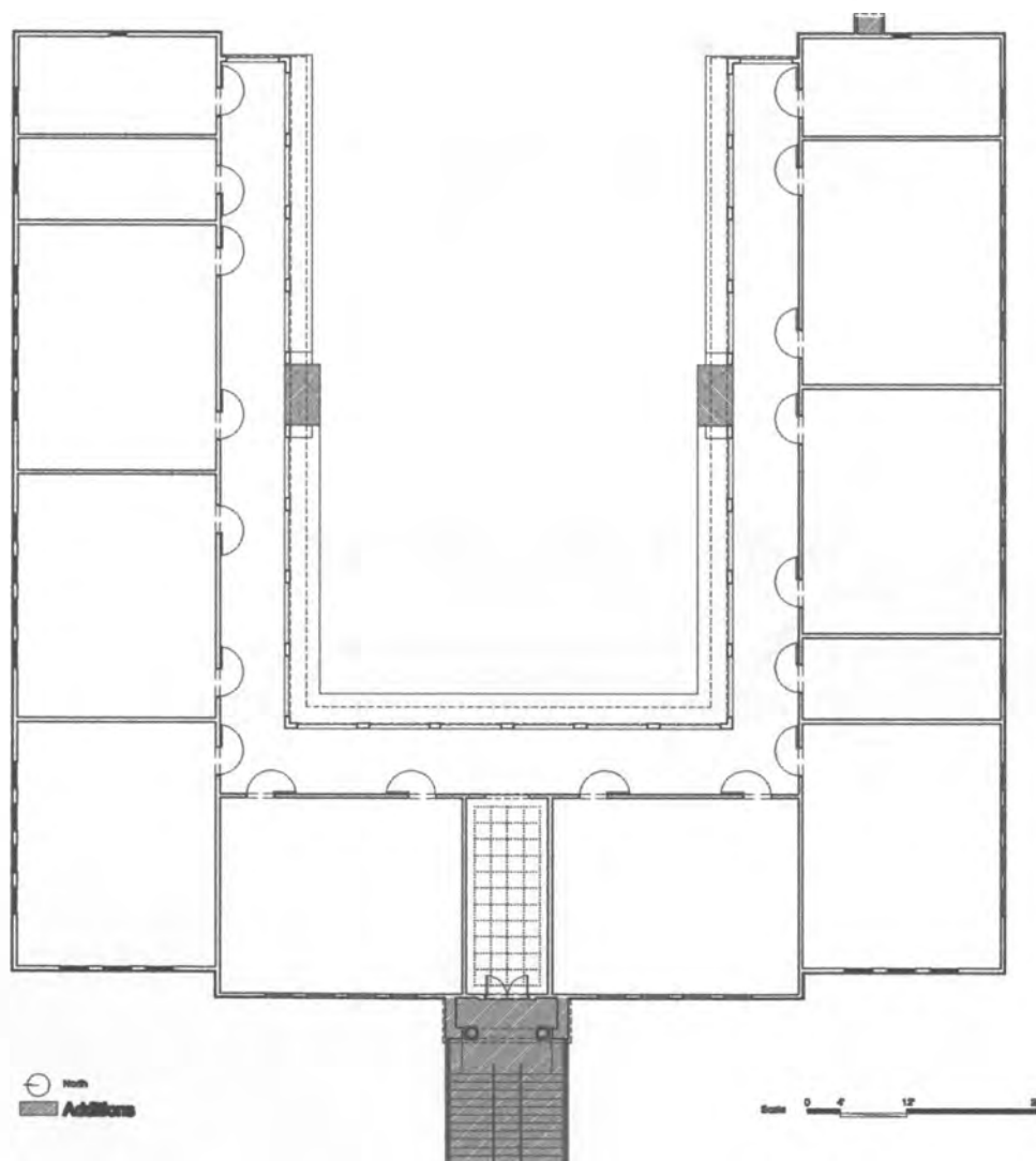
FIG. 2: Luis Muñoz Rivera School, in Lajas Puerto Rico, U-shaped volume. It includes eight classrooms, one office, one storage area, two restrooms, and corridors, all enclosed within a 120 feet x 115 feet perimeter. Drawing: Eduardo Miranda, August 25, 2012. Source: Jorge Rigau Arquitectos, San Juan Puerto Rico.
