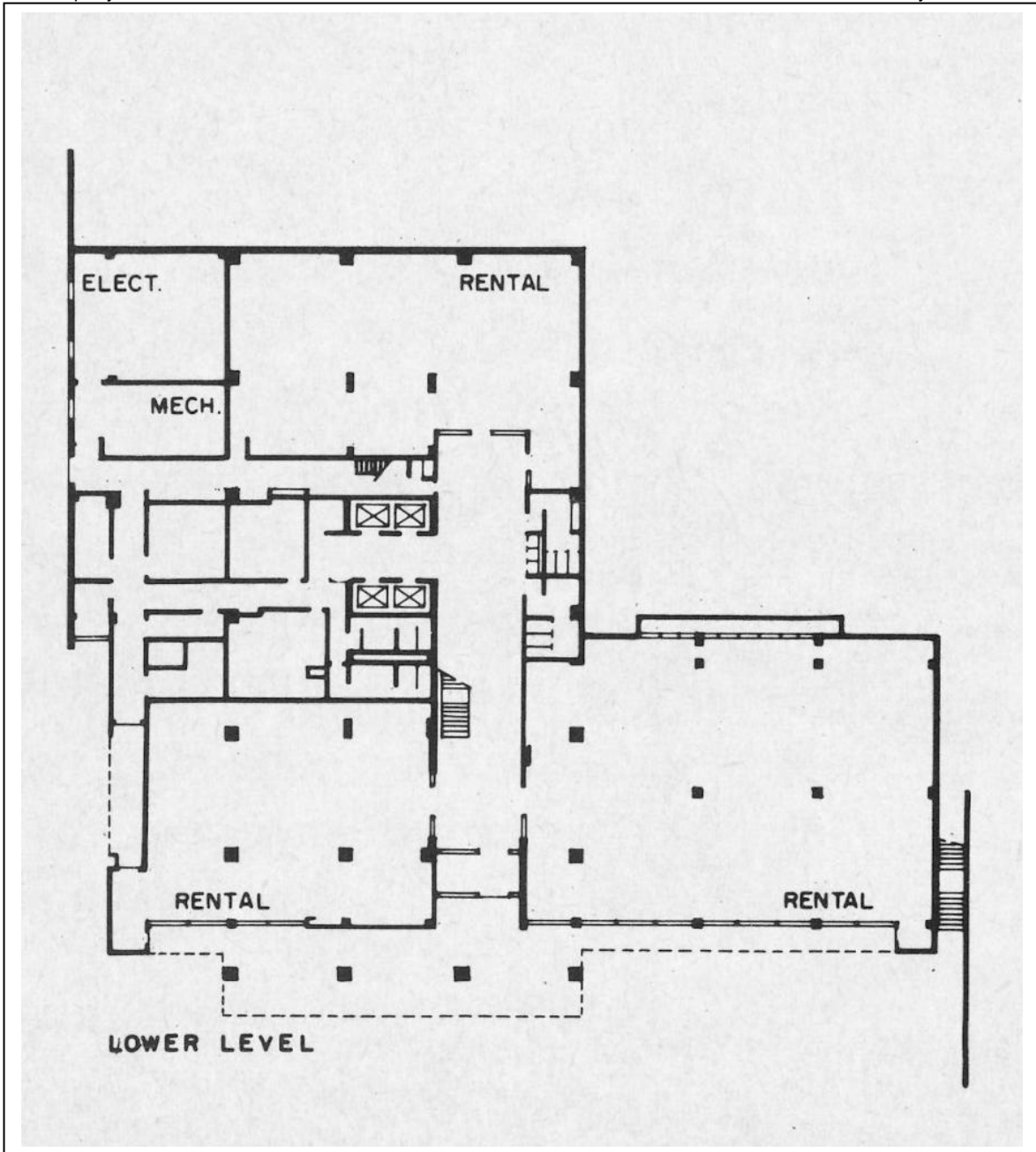
Figure 9: Lower Level Plan, 1968 Architectural Record, March 1969
