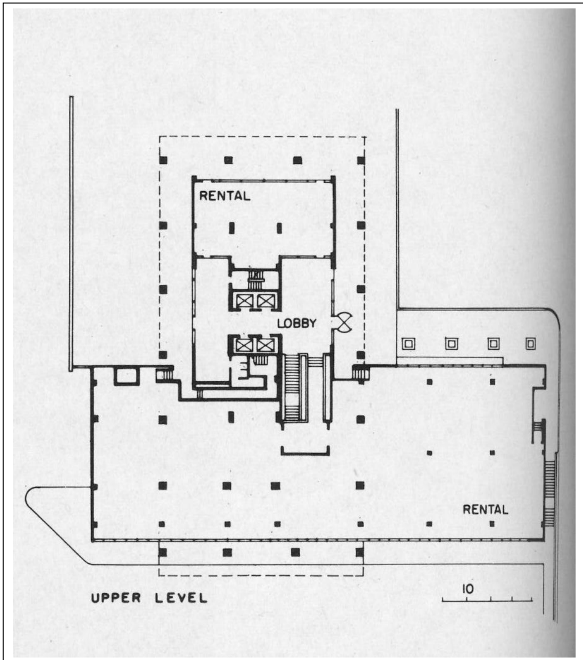
Figure 10: First Floor Plan, 1968 Architectural Record, March 1969
