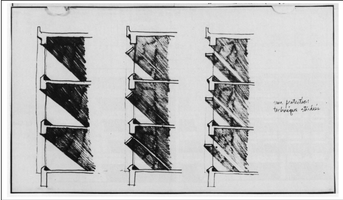
Figure 5: Sun Protection Technique Studies, 1964 The Walter Gropius Archive, Volume Four
