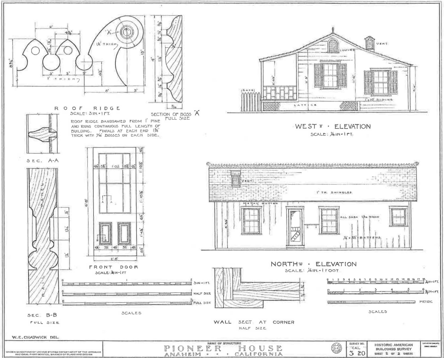
Figure 6: HABS Drawing Sheet 2, 1934.
