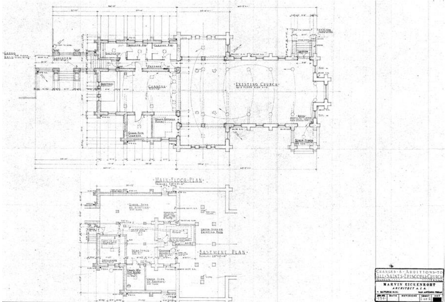
Figure 14: Drawings, Marvin Eickenroht, AIA, 1939.
