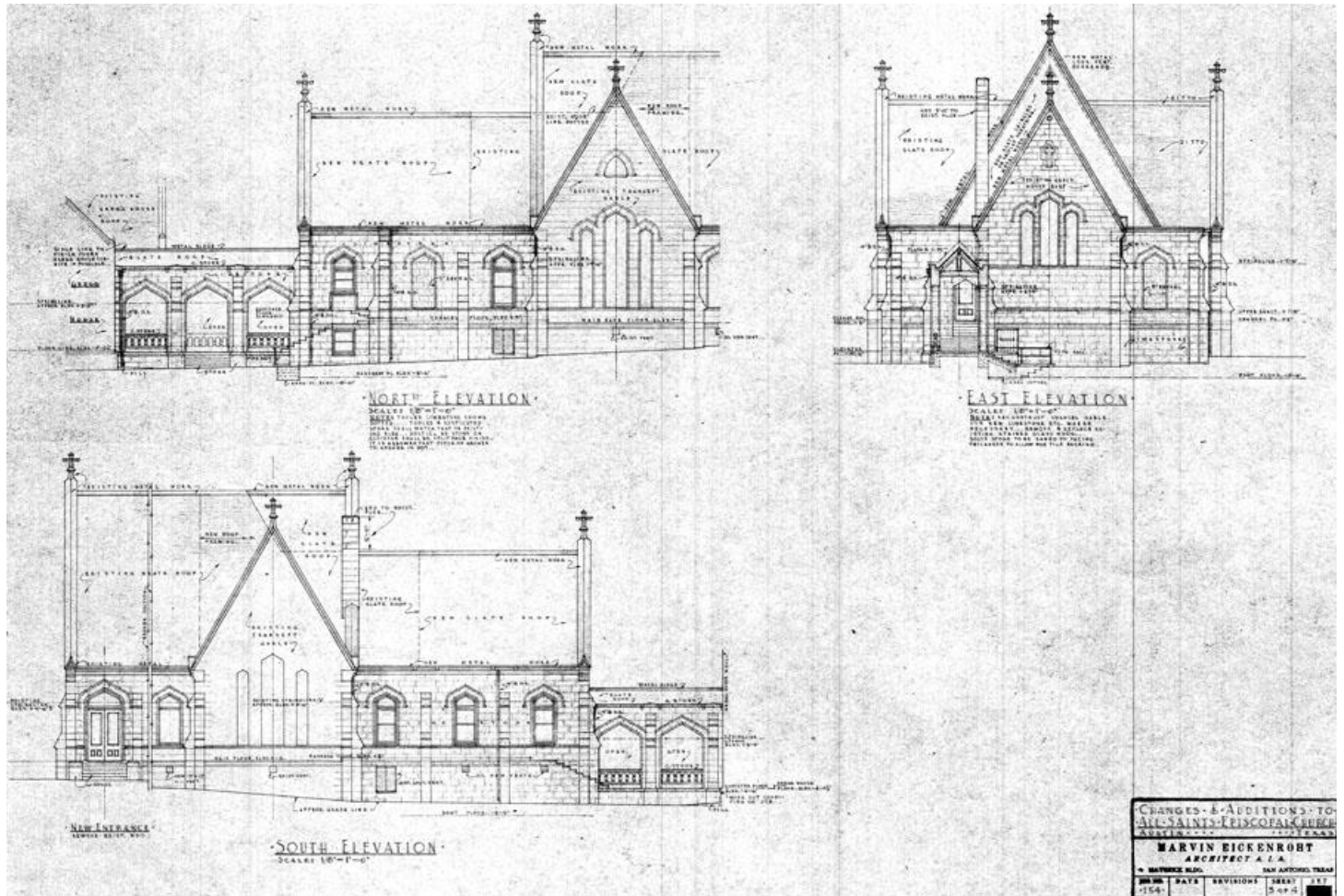
Figure 15: Elevations, 1939, Marvin Eickenroht, AIA.
