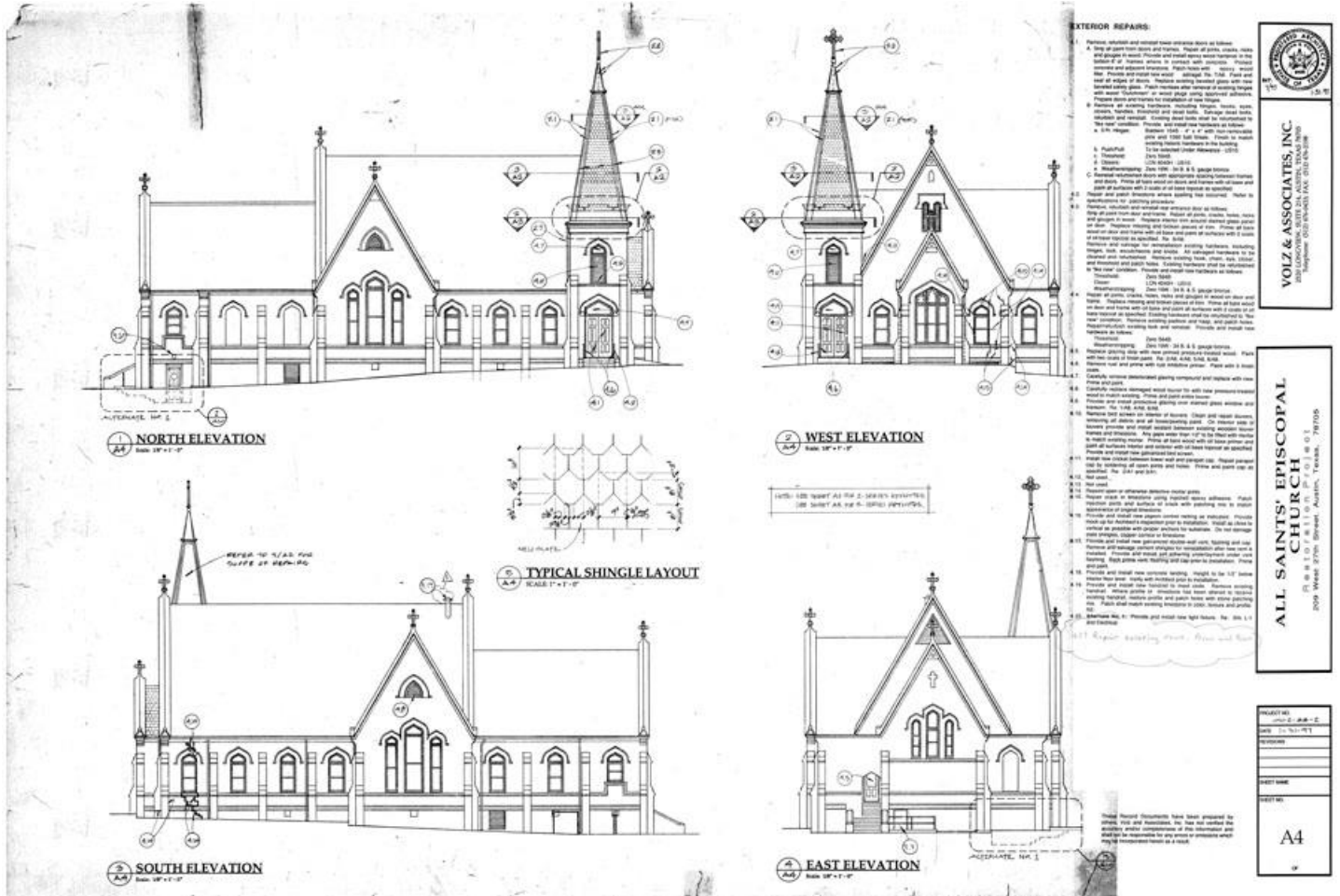
Figure 17: Elevations prepared by Volz & Associates, Inc., 1997, for preservation project.
