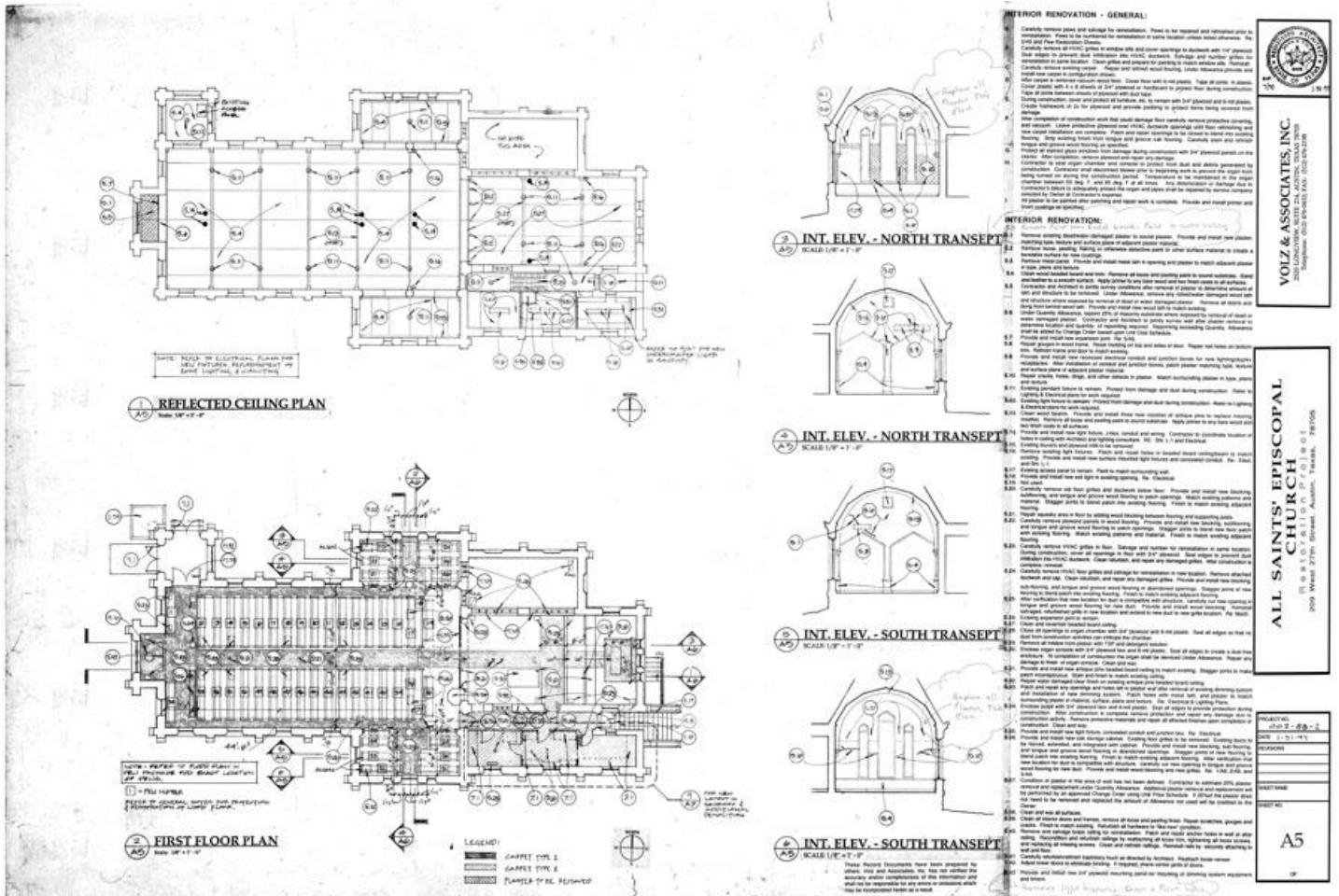
Figure 18: First floor plan, reflected ceiling plan, and selected interior elevations. Prepared by Volz & Associates, Inc., 1997.
