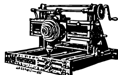
LOCOMOTIVE PORT MILLING MACHINE.
