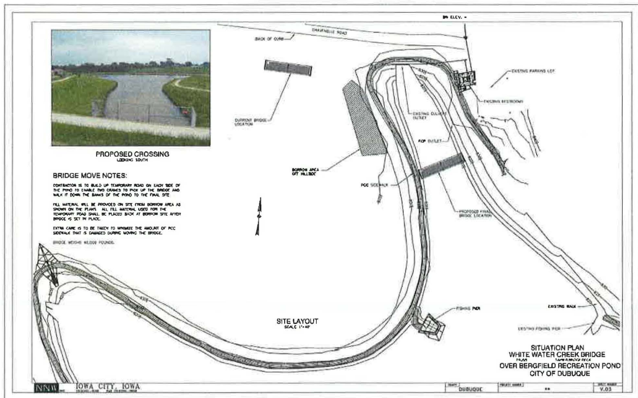
Fig. 4 Situation Plan – White Water Creek Bridge over Bergfield (sic) Recreation Pond.
