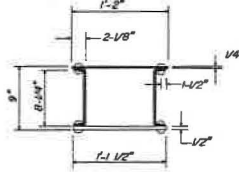
STRUT AT CENTER OF FIRST OPENING FROM UPPER CHORD
