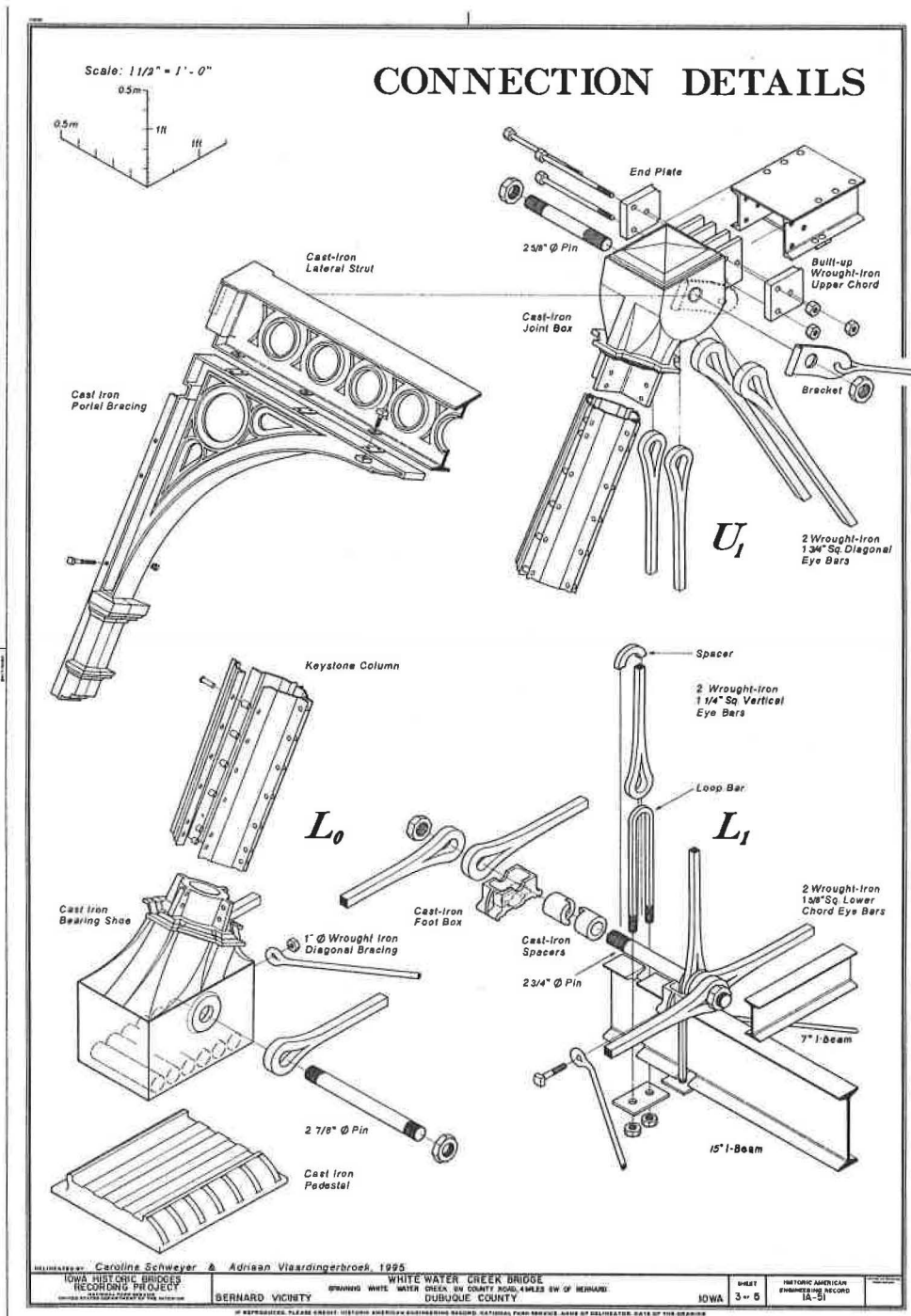
Fig. 7 Historic American Engineering Record drawing, 1995
