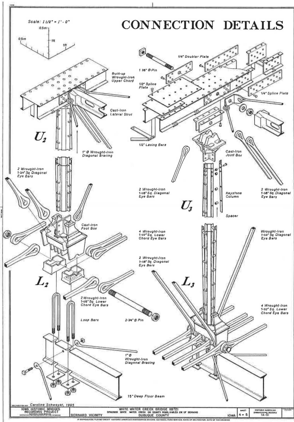
Fig. 8 Historic American Engineering Record drawing, 1995
