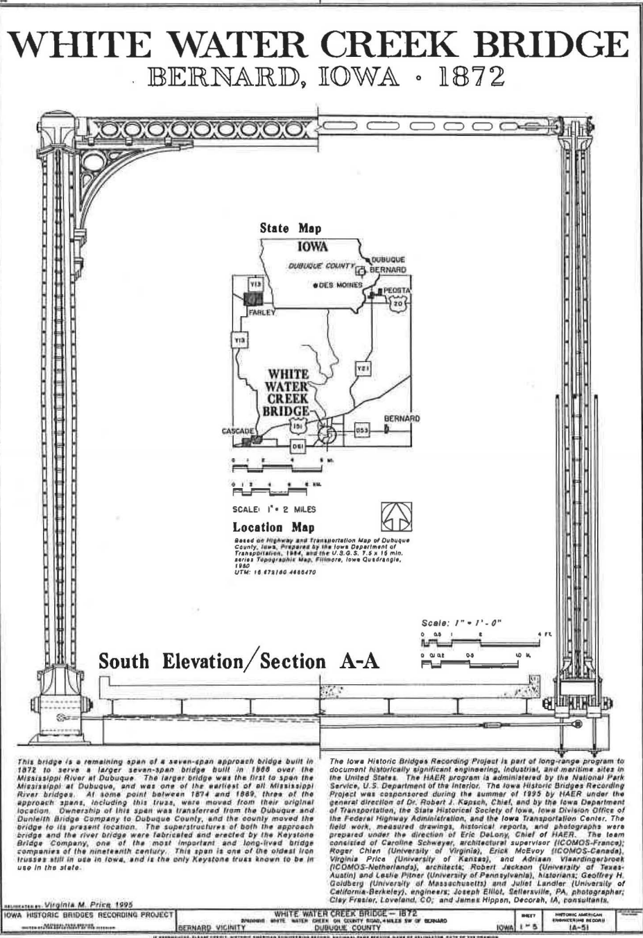
Fig. 5 Historic American Engineering Record drawing, 1995
