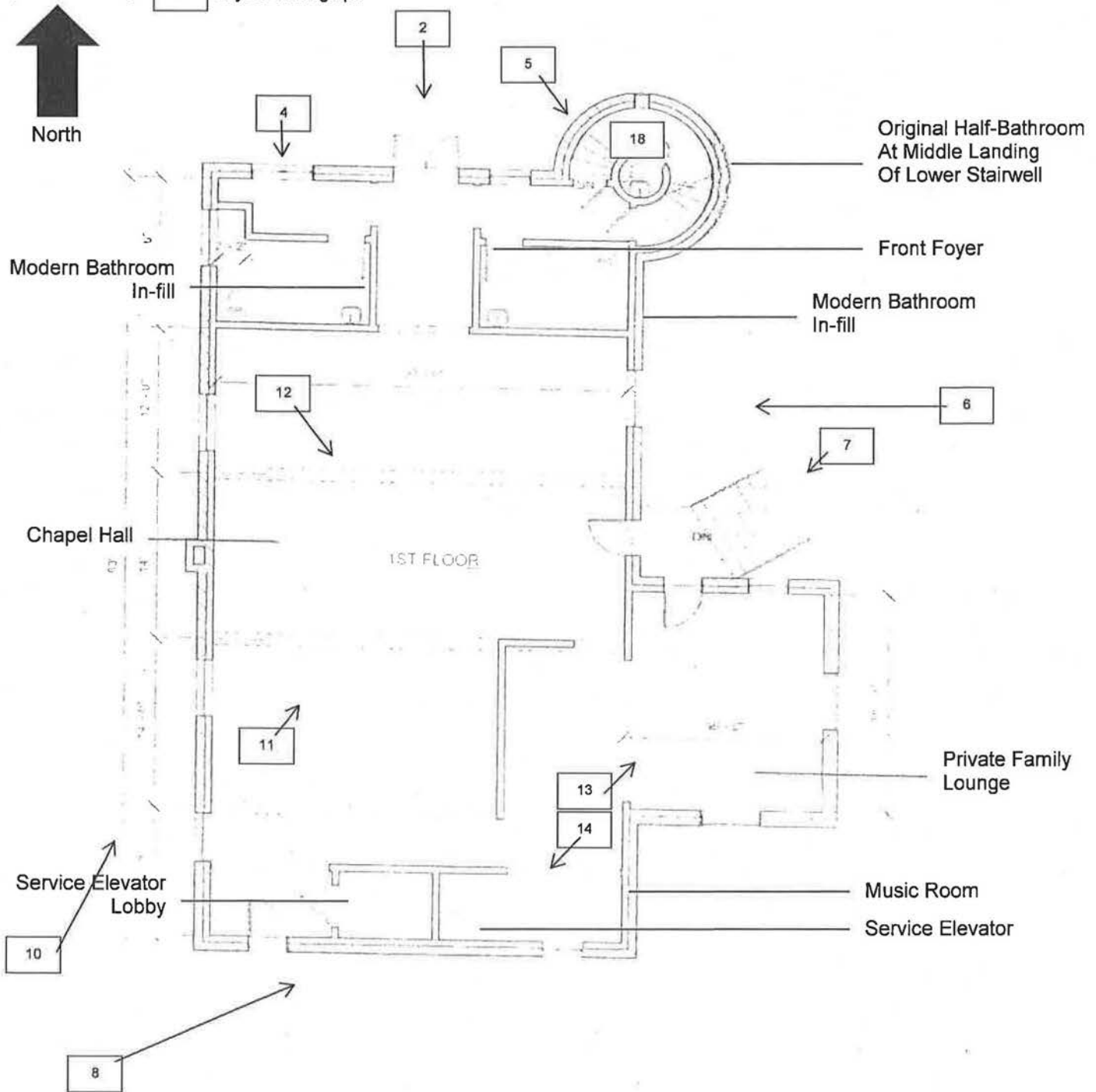
Figure 3: Sketch Plan. First Floor
