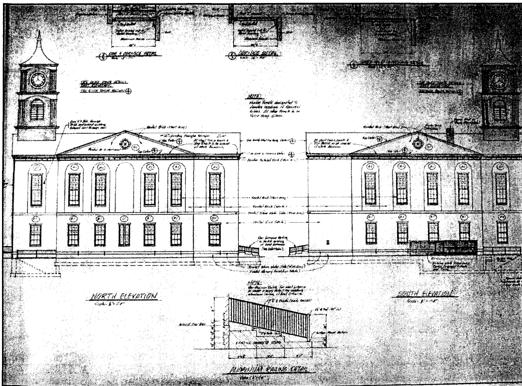
Figure 8c: Elevations from Barth drawings, 1999.
