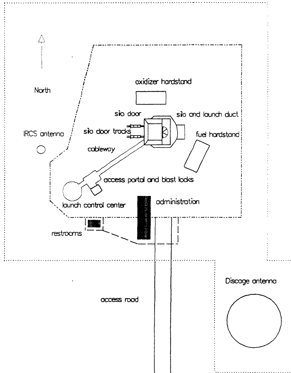
Figure #1 Titan II ICBM Missile Site 8 (571-7) Green Valley, Pima Co., Arizona Site layout. David K. Stumpf, 1993
