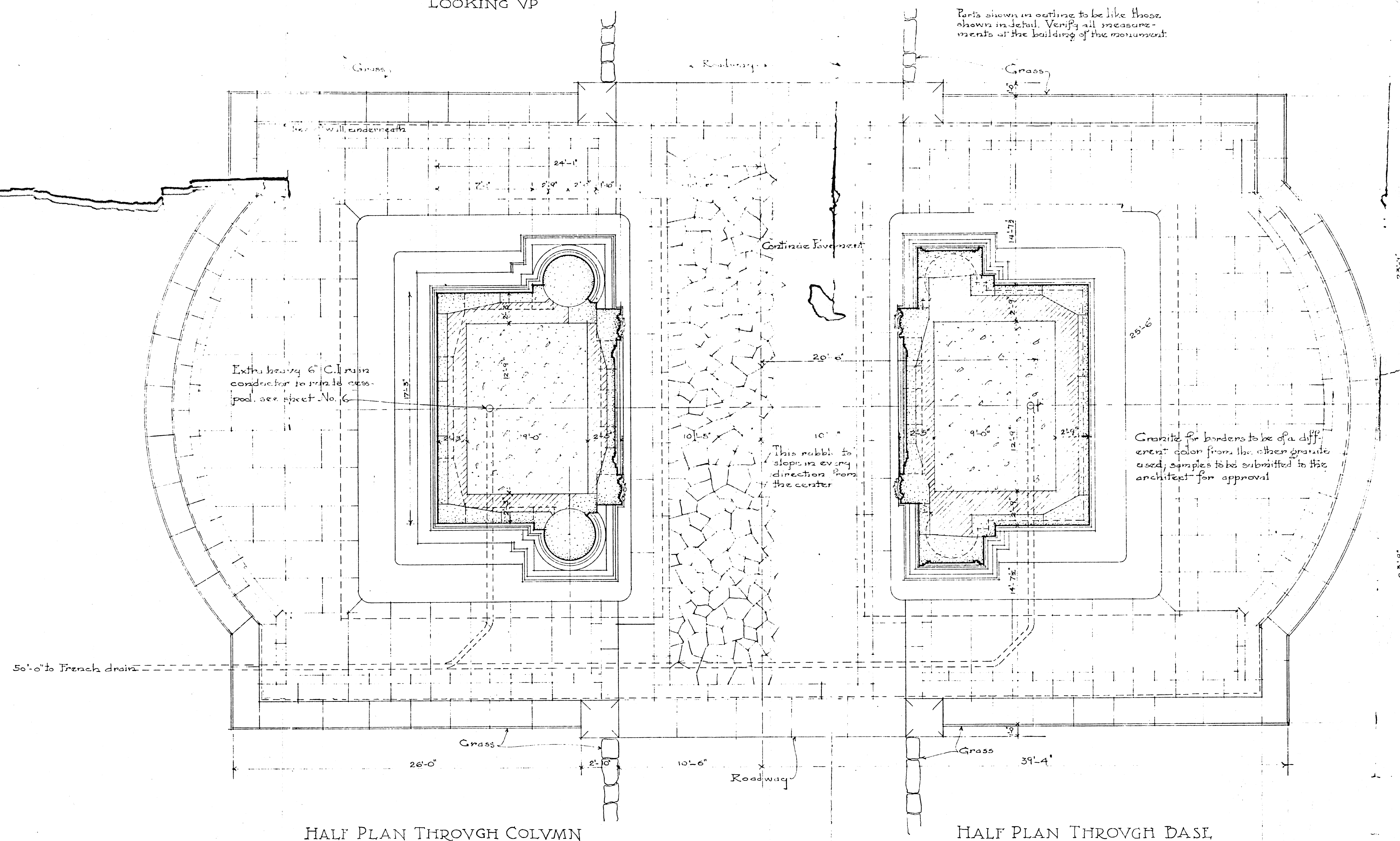
HALF PLAN OF ROOF
