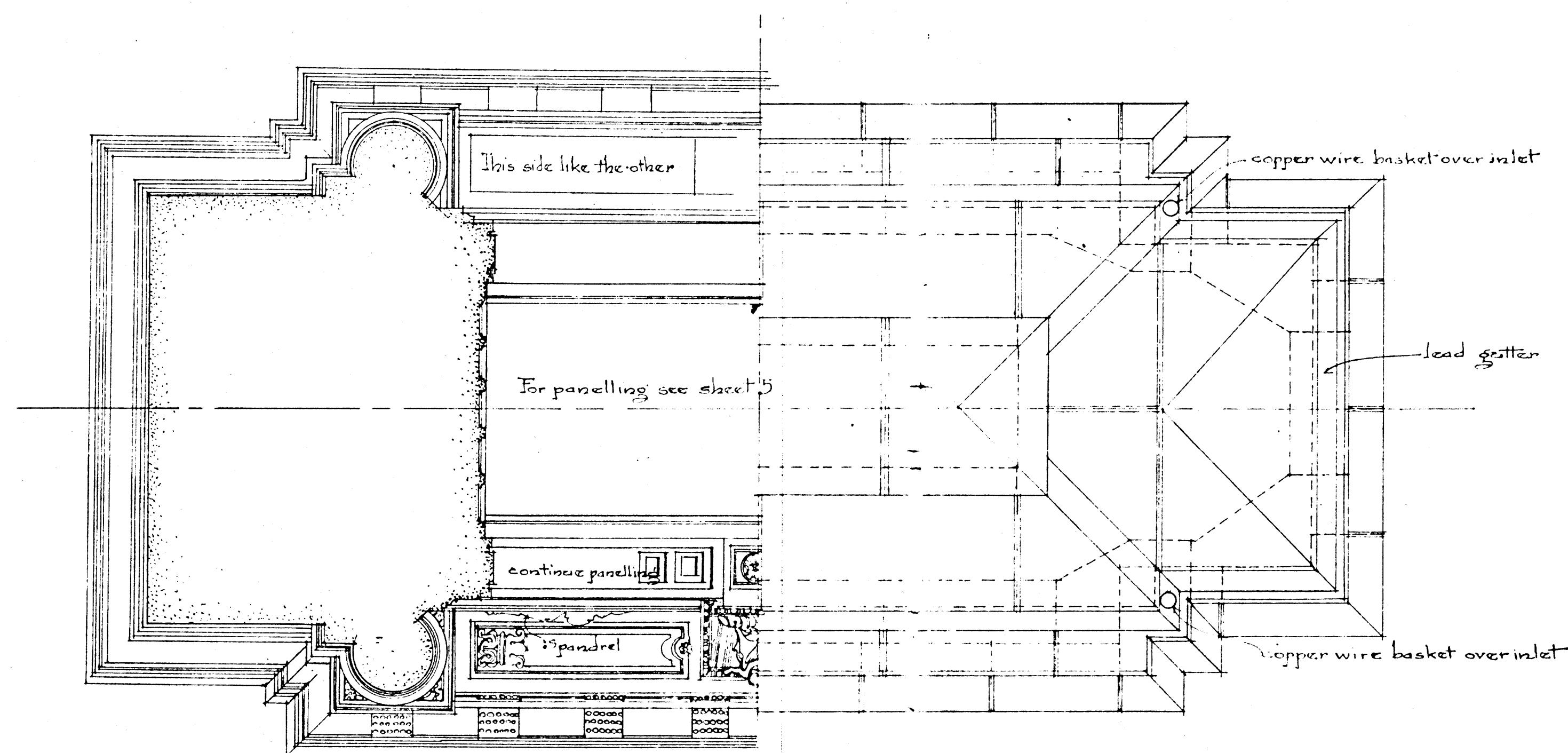
HALF PLAN AT LEVEL OF CENTER OF ARCH LOOKING UP
