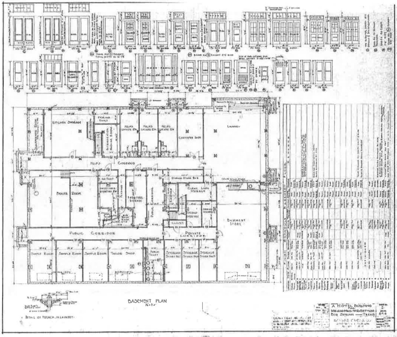
FIGURE 1: Original plan, basement level.
