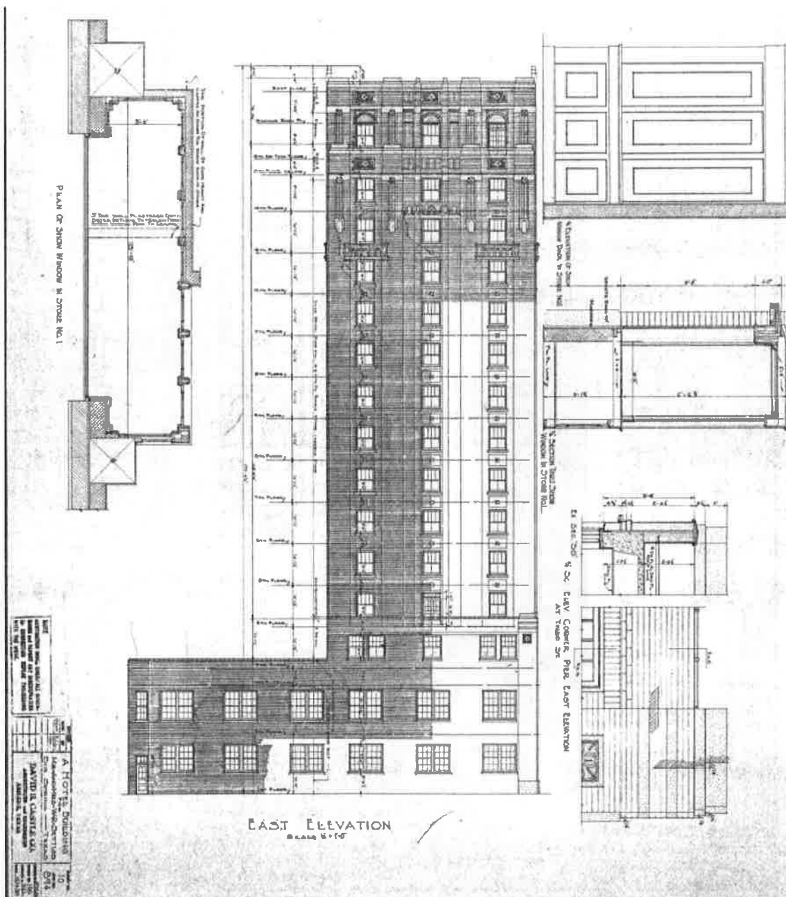
FIGURE 9: Original east elevation and details.
