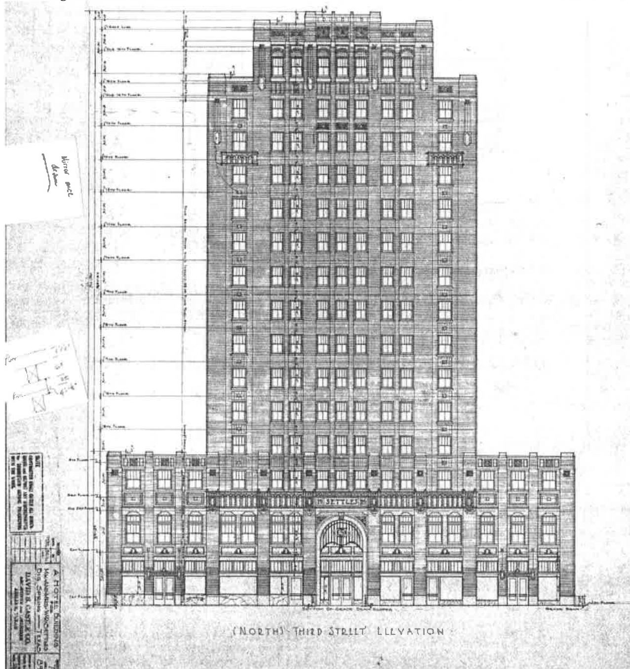
FIGURE 6: Original north elevation.
