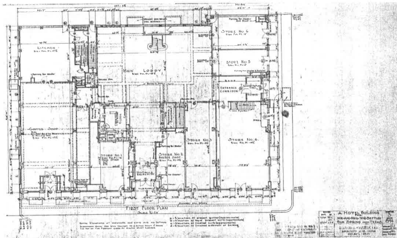
FIGURE 2: Original plan, first floor.
