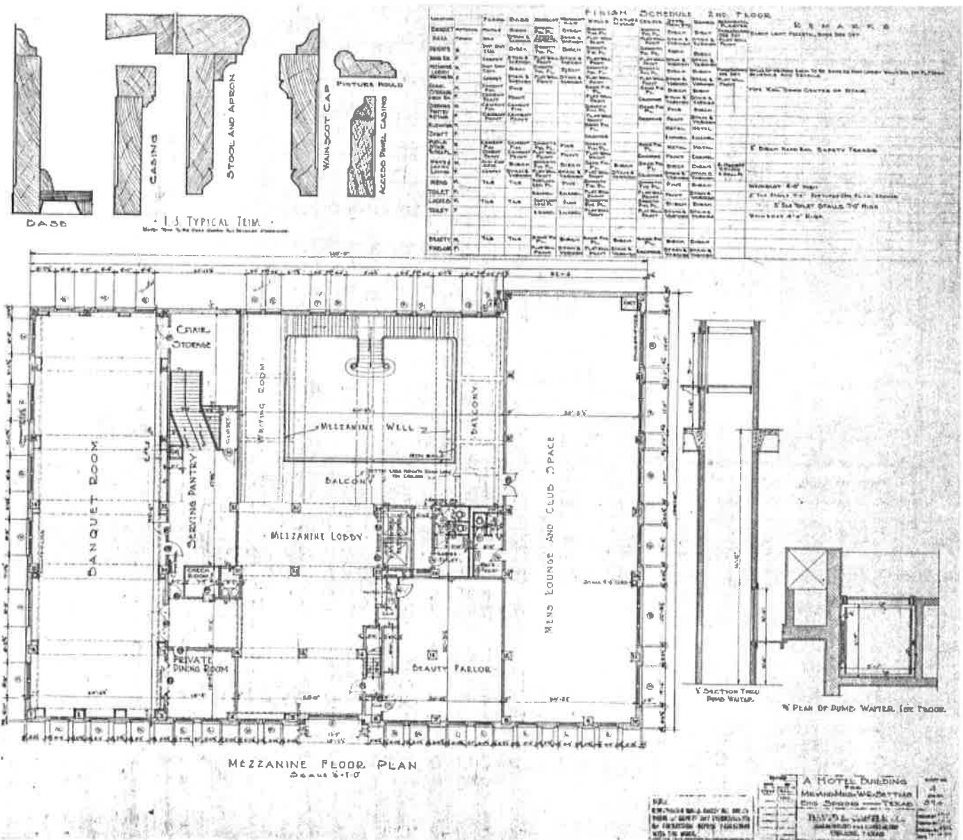
FIGURE 3: Original plans and details, mezzanine.
