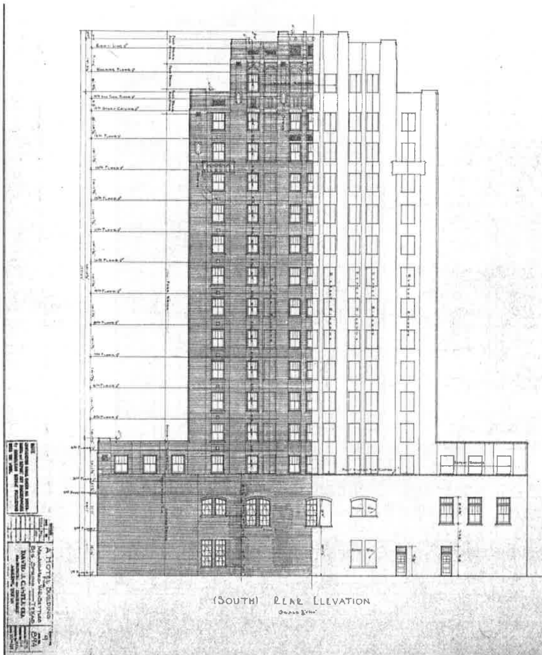
FIGURE 7: Original south elevation.
