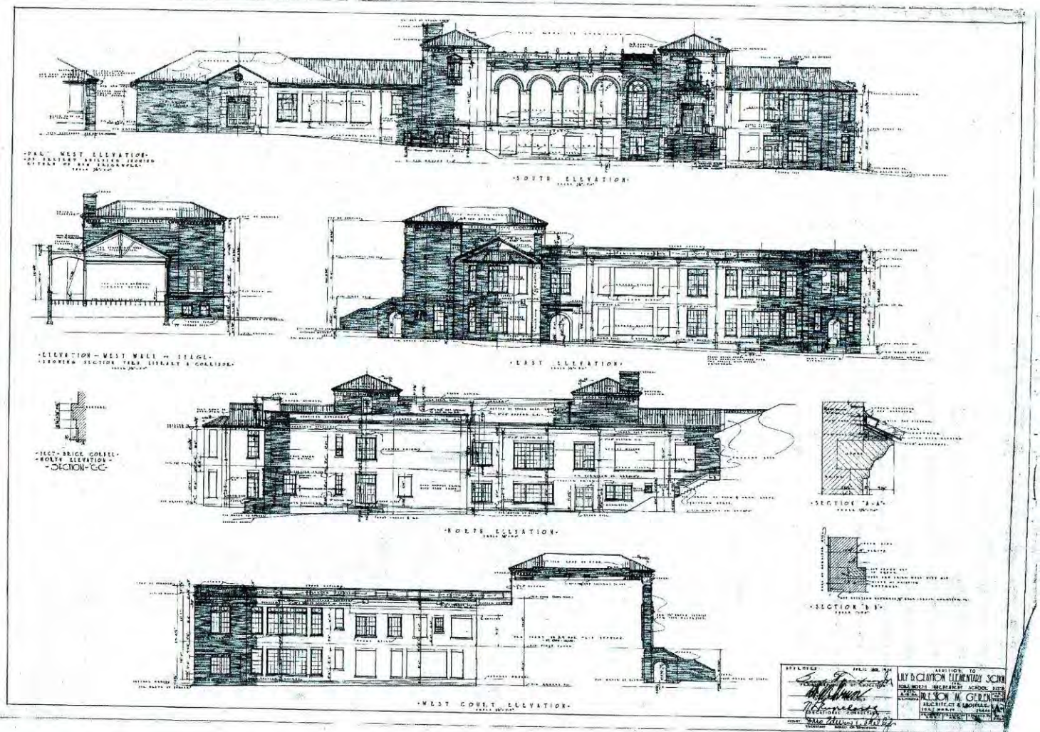
Figure 15: Elevations of the 1934-1935 addition beginning at the top with the south elevation followed by the east, north, and west elevations. Preston M. Geren, Architect. Courtesy Lily B. Clayton Archives.
