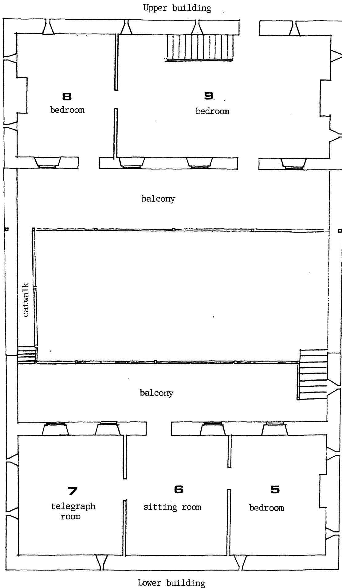
4.(b) SECOND FLOOR PLAN.
