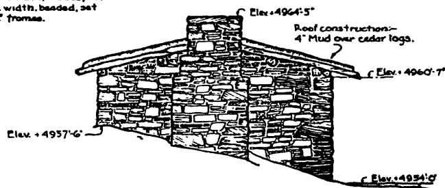
SOUTH ELEVATION
