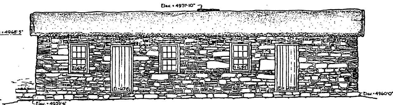
SOUTH ELEVATION
