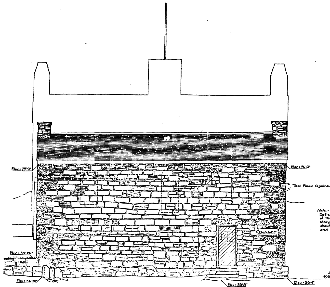
FRONT (SOUTHEAST) ELEVATION
