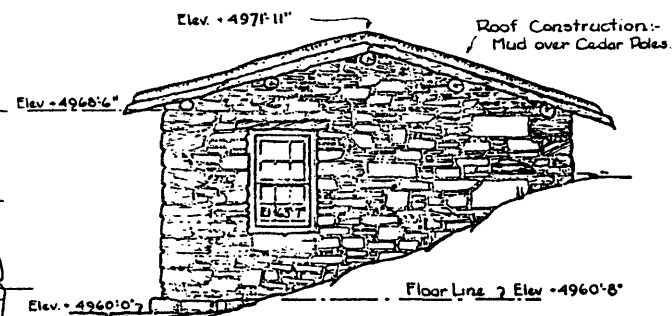
EAST ELEVATION
