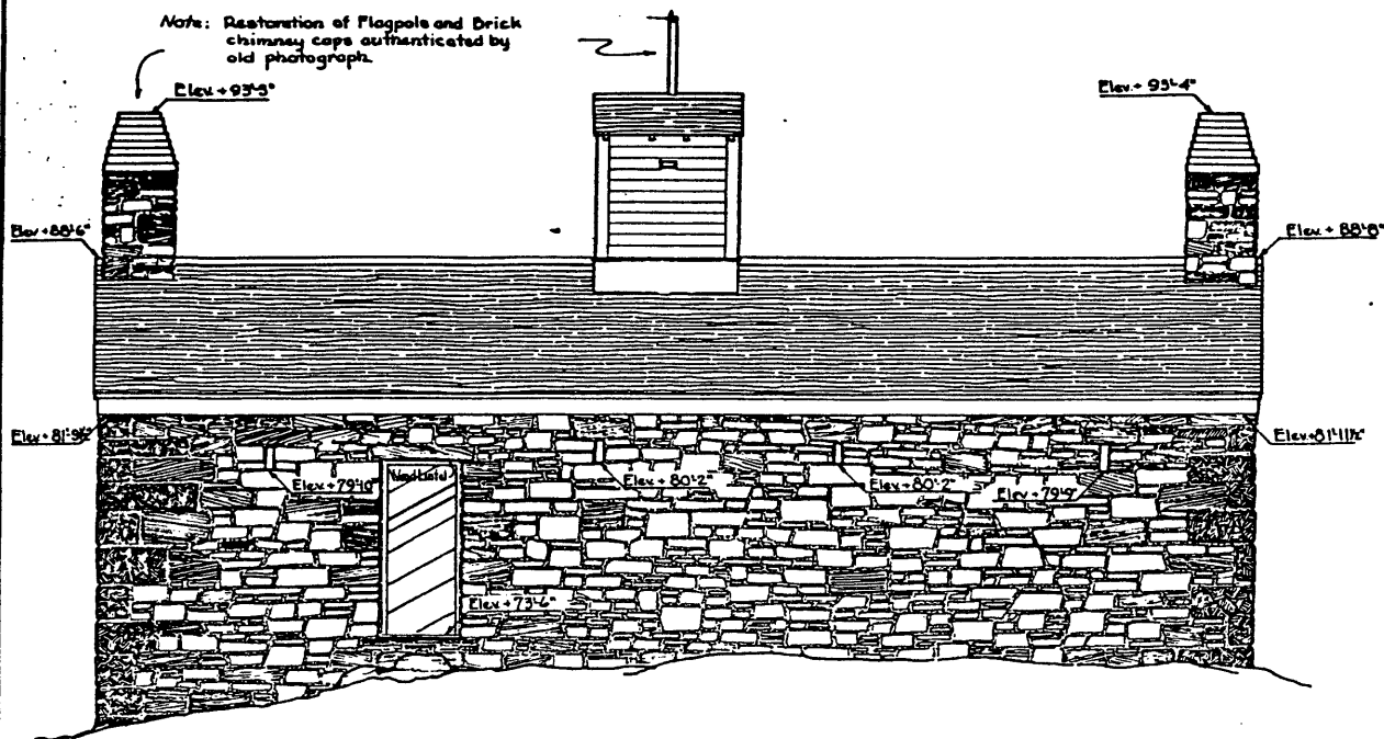
NORTHWEST ELEVATION
