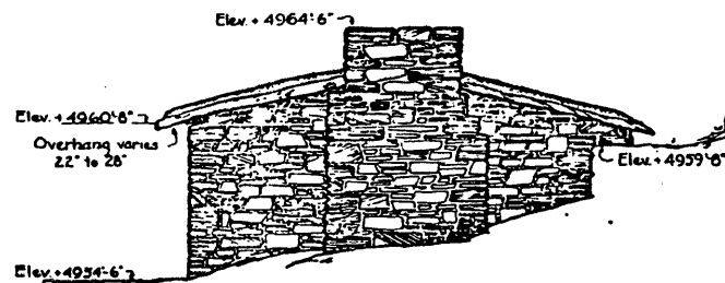
NORTH ELEVATION
