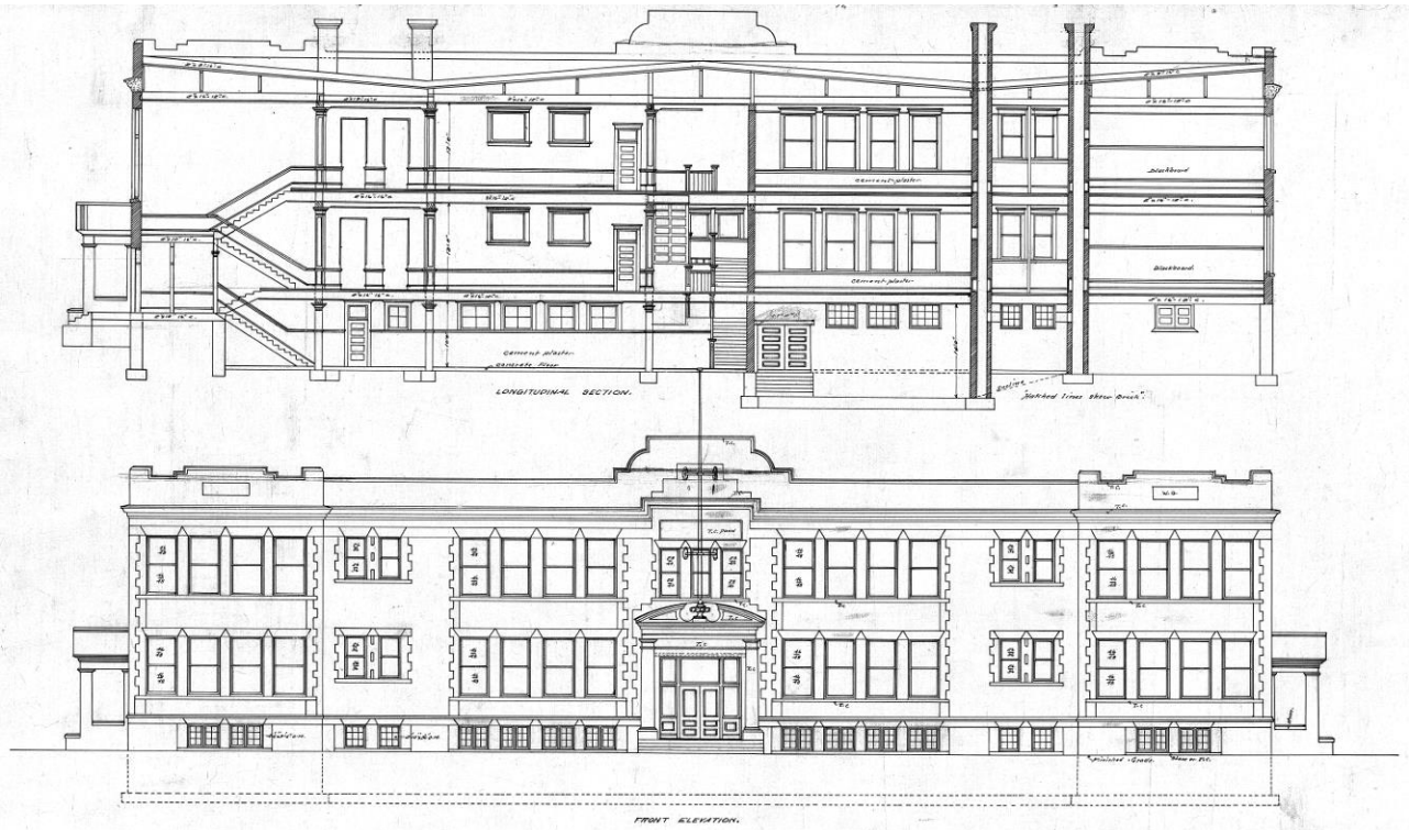
FRONT ELEVATION.
