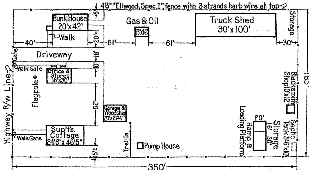
TYPICAL MAINTENANCE STATION LAYOUT
