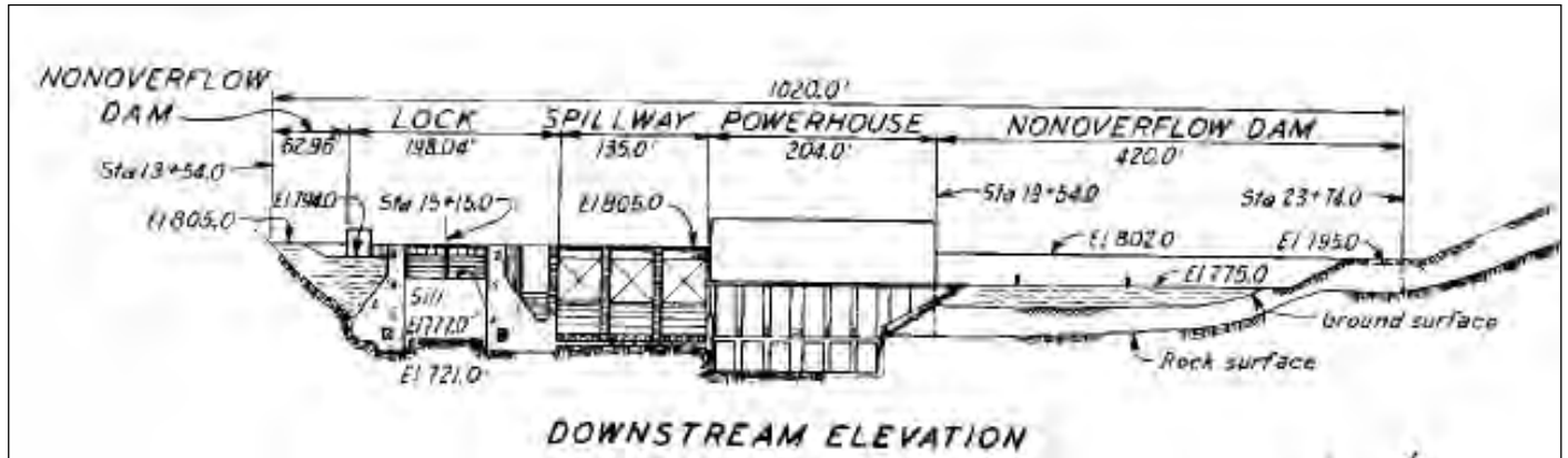
Downstream Elevation of Melton Hill Hydroelectric Project
