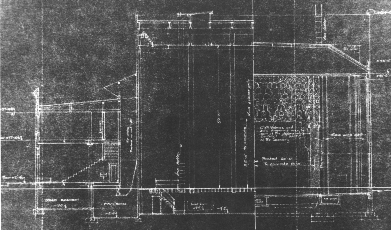
PROSCENIUM AND CROSS SECTION OF AUDITORIUM Scale \frac{1}{8}'' = 1'-0''
