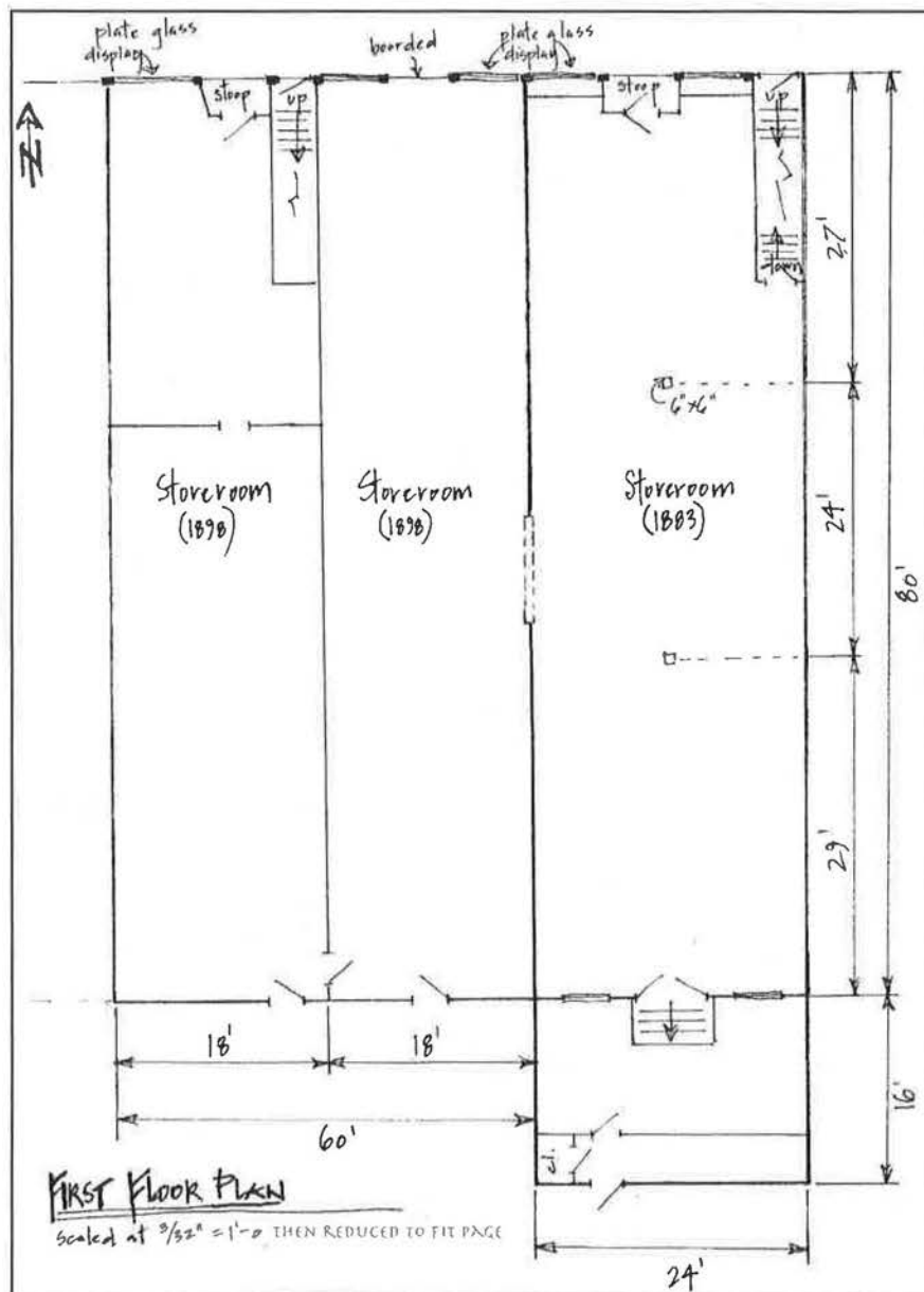
Figure 3. FIRST FLOOR PLAN – 2013
