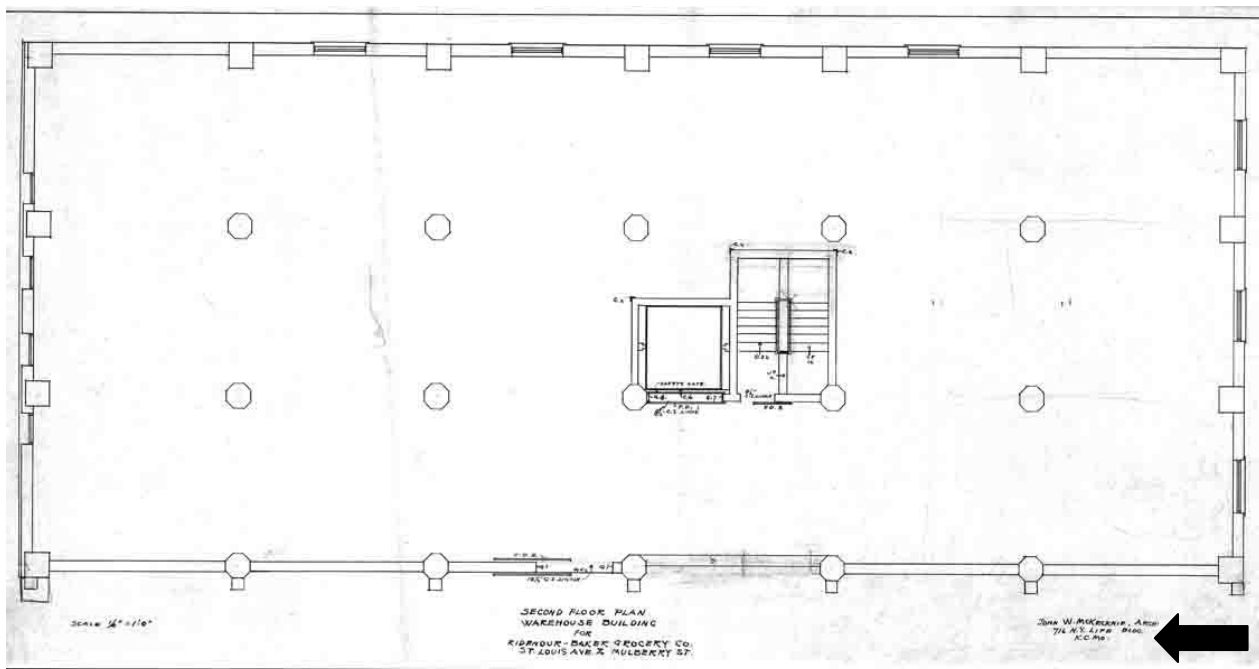
Figure 13: Historic Plans, 1910 block, typical upper floor plan. Source: The State Historical Society of Missouri, Kansas City.
