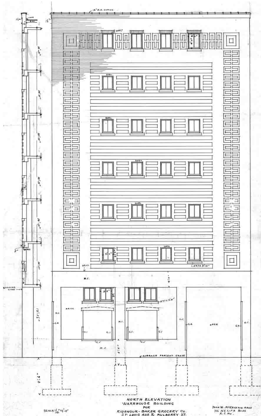
Figure 11: Historic Plans, 1910 block, north elevation. Source: The State Historical Society of Missouri, Kansas City.
