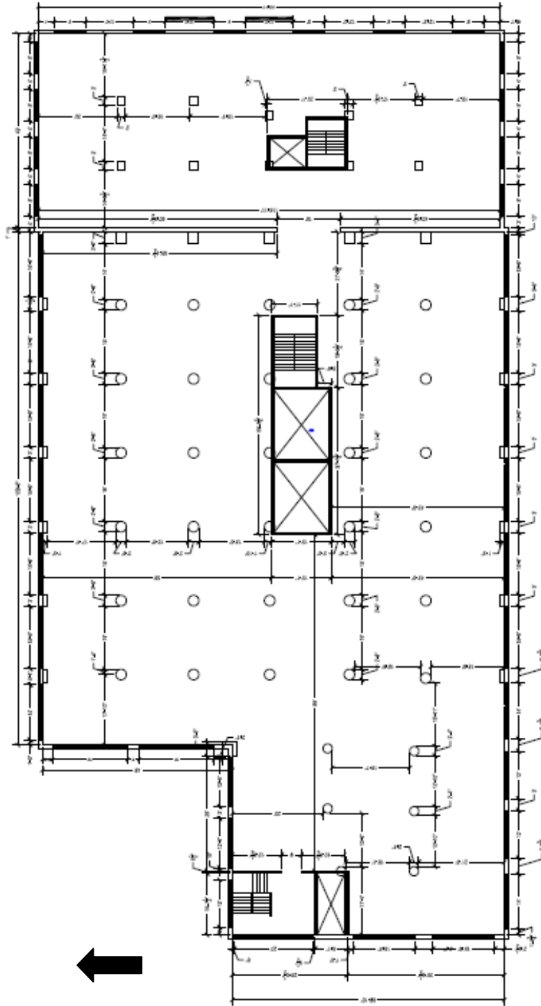
Figure 14: Existing floorplan, typical interior, 1910 and 1915 block.
