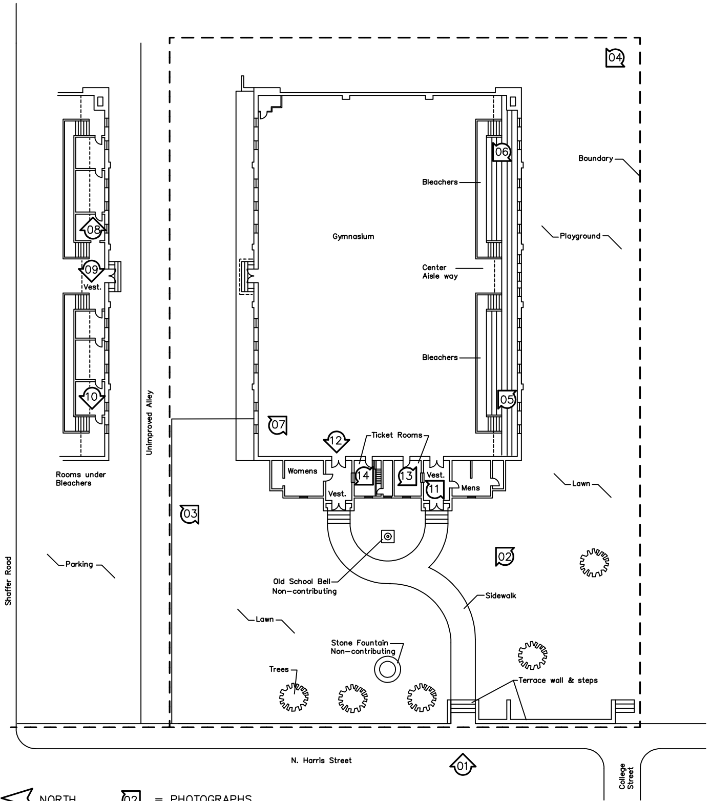
BOURBON COMMUNITY BUILDING-GYMNASIUM NATIONAL REGISTER SITE & MAIN LEVEL PLAN
