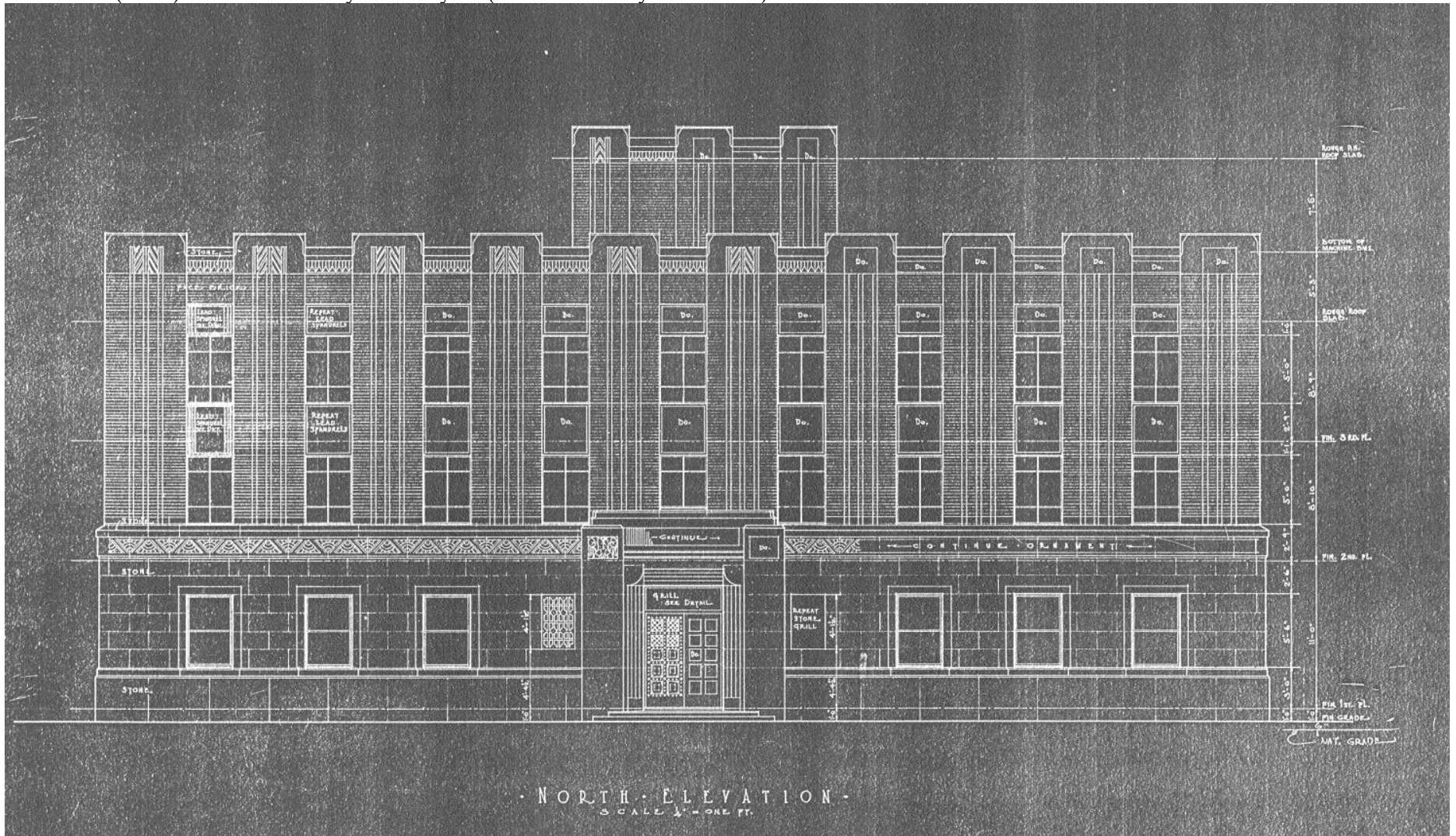
1931 North (Front) Elevation Plans by S. B. Haynes (Lubbock County Courthouse)
