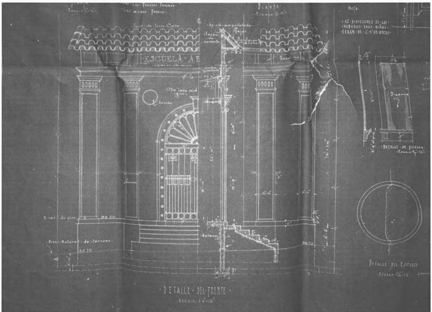
Main entrance detail drawings for the José Fontán School designed by architect Joseph O'Kelly. Source: AGPR Fondo Obras Públicas, Edificios Escolares. Caja: 1140, Legajo, 205, Exp. 1
