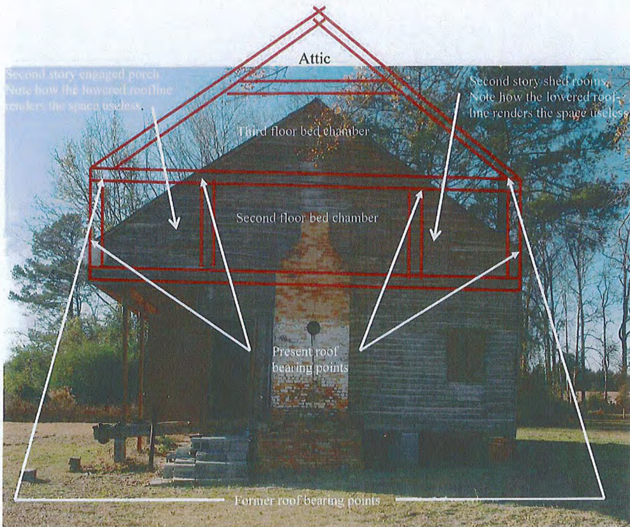
Diagram showing the ca. 1853 remodeling of the Carter-Simmons House 31
