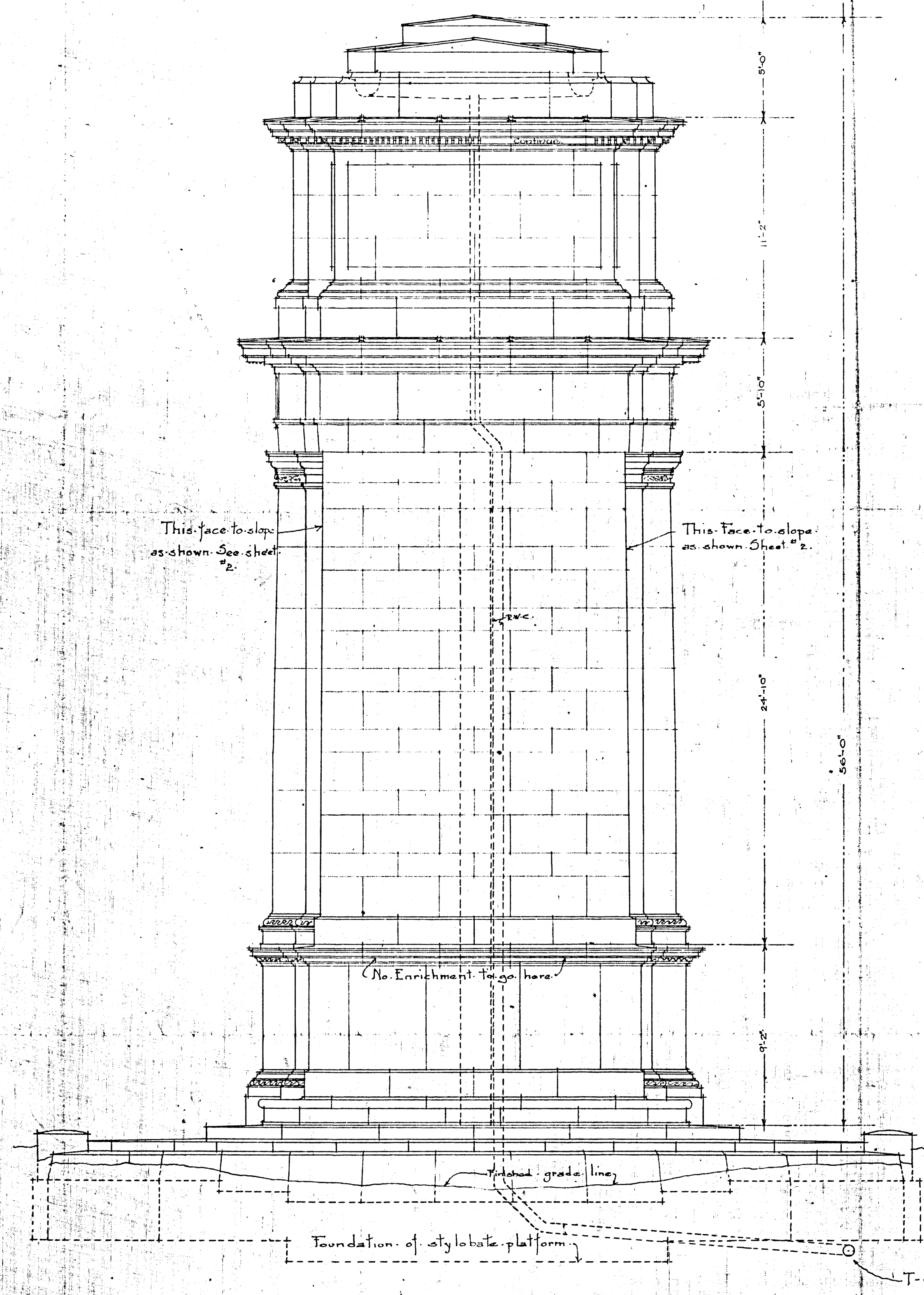
EAST - ELEVATION WEST-ELEVATION - SIMILAR.
