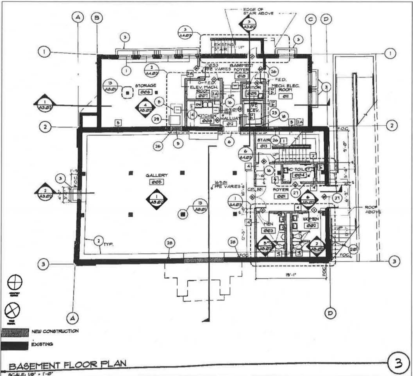
Figure 7: Renovated Basement Floor Plan, Slusarenko Architecture, PC, 2001.
