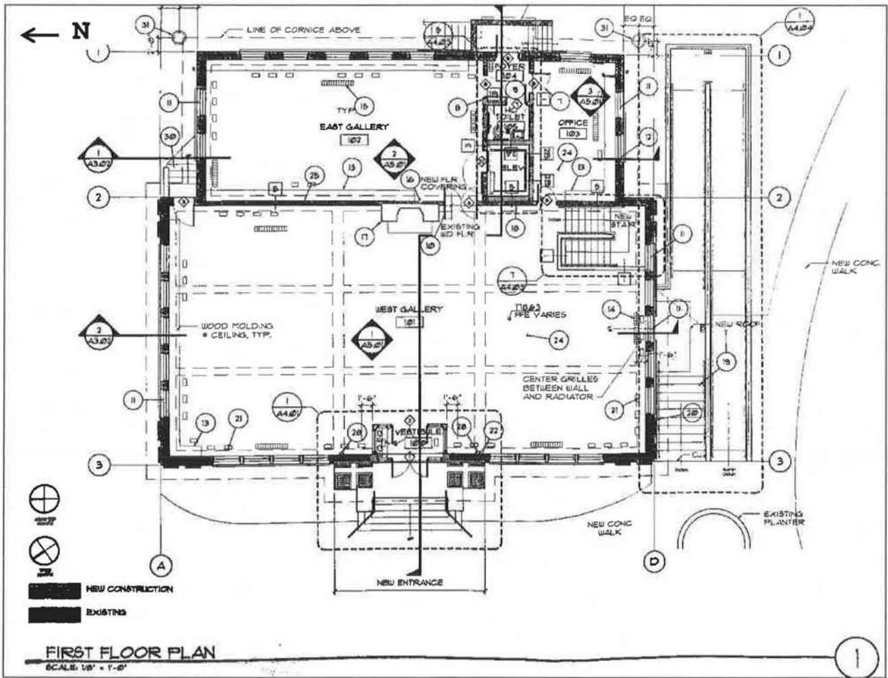
Figure 6: Renovated First Floor Plan, Slusarenko Architecture, PC, 2001.
