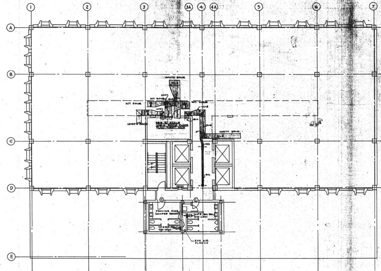
TYPICAL FLOOR PLAN SCALE 1/8" = 1'-0"
