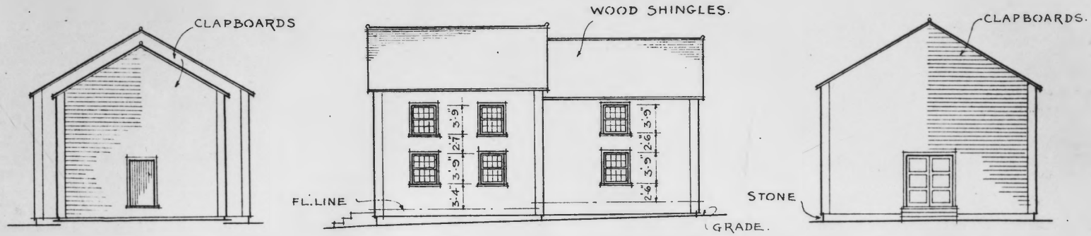
EAST ELEV. SCALE \frac{1}{8}'' = 1'-0'' SOUTH ELEVATION SCALE \frac{1}{8}'' = 1'-0'' WEST (FRONT) ELEV.
