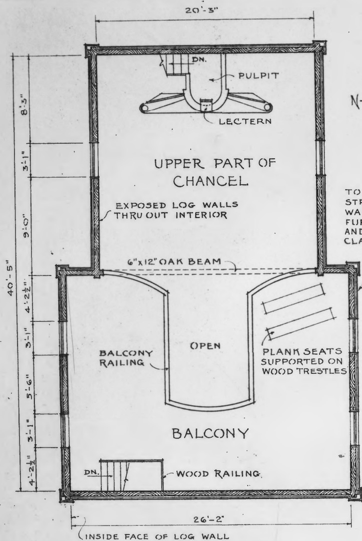
BALCONY PLAN
