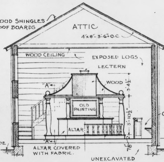
SECTION THRU CHANCEL TOWARD ALTAR SCALE \frac{1}{4}'' = 1'-0''
