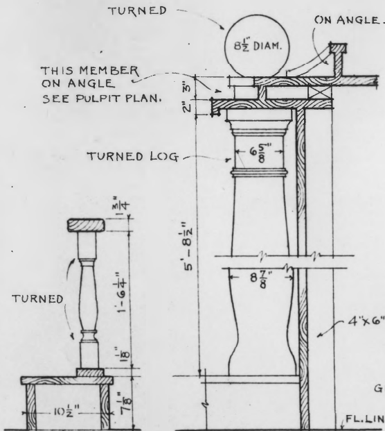
SEC "A-A" SCALE \frac{1}{2}'' = 1'-0''
