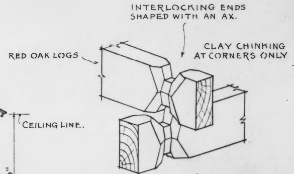
ISOMETRIC VIEW SHOWING METHOD OF INTERLOCKING LOGS AT CORNERS OF BUILDING.
