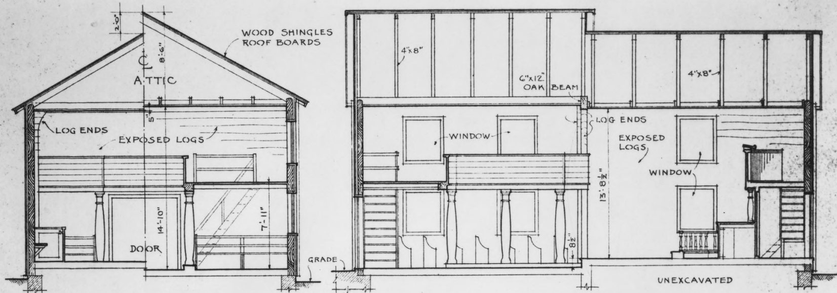
SECTION ON LINE - "A-B" SCALE \frac{1}{4}'' = 1'-0'' LONGITUDINAL SECTION ON \odot OF BLDG.
