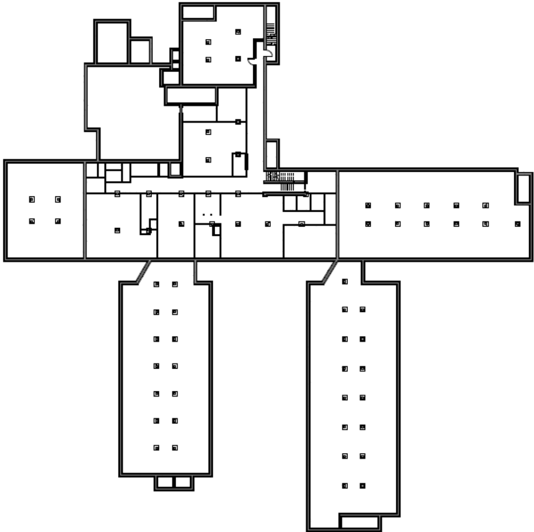
Existing Floor Plan, Basement. (NE45 Architecture, "Preliminary Architectural Report," 12).
