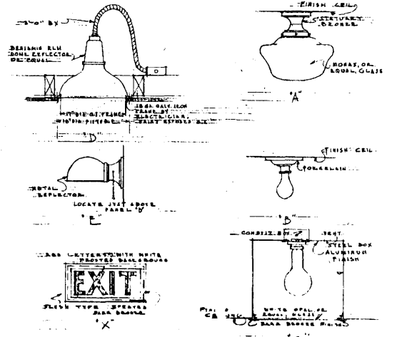
ELECTRIC FIXTURES NOT TO SCALE SIZE OF FIXTURES DETERMINED BY SIZE OF LIGHTS REQUIRED
