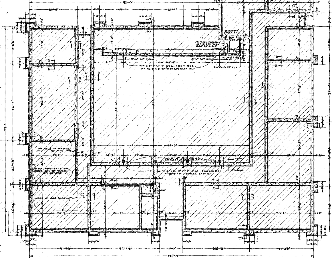
FOOTING AND FOUNDATION PLAN SCALE 1/4" = 1'-0"
