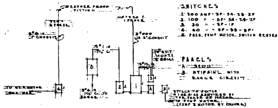
ELECTRIC DIAGRAM NOT TO SCALE
