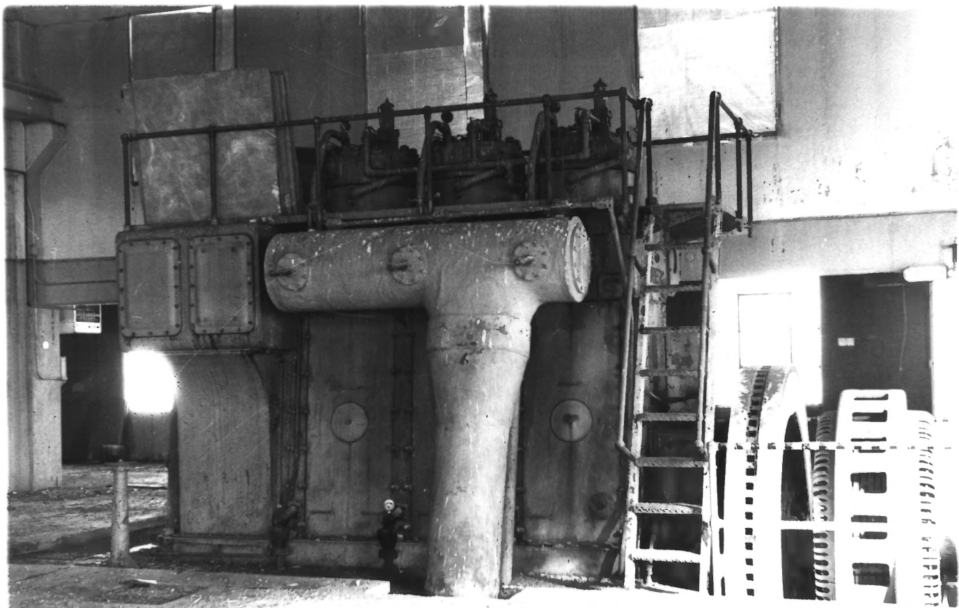
REAPLANT - Franklin Co. Iowa - Item VI Photo B. Inside building. Engines and generator.
