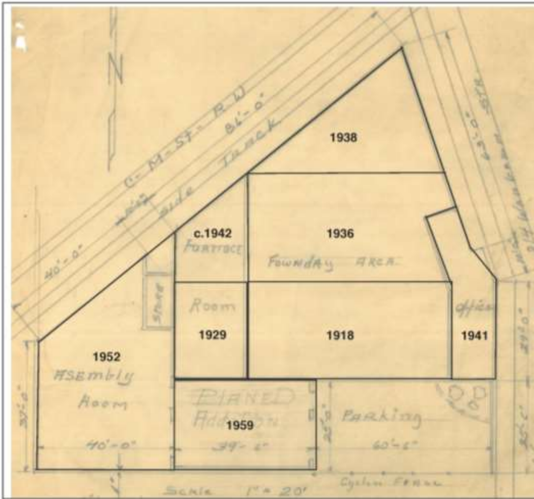
Figure 4. Madison Brass Works, Plan with Construction Dates Not to scale
