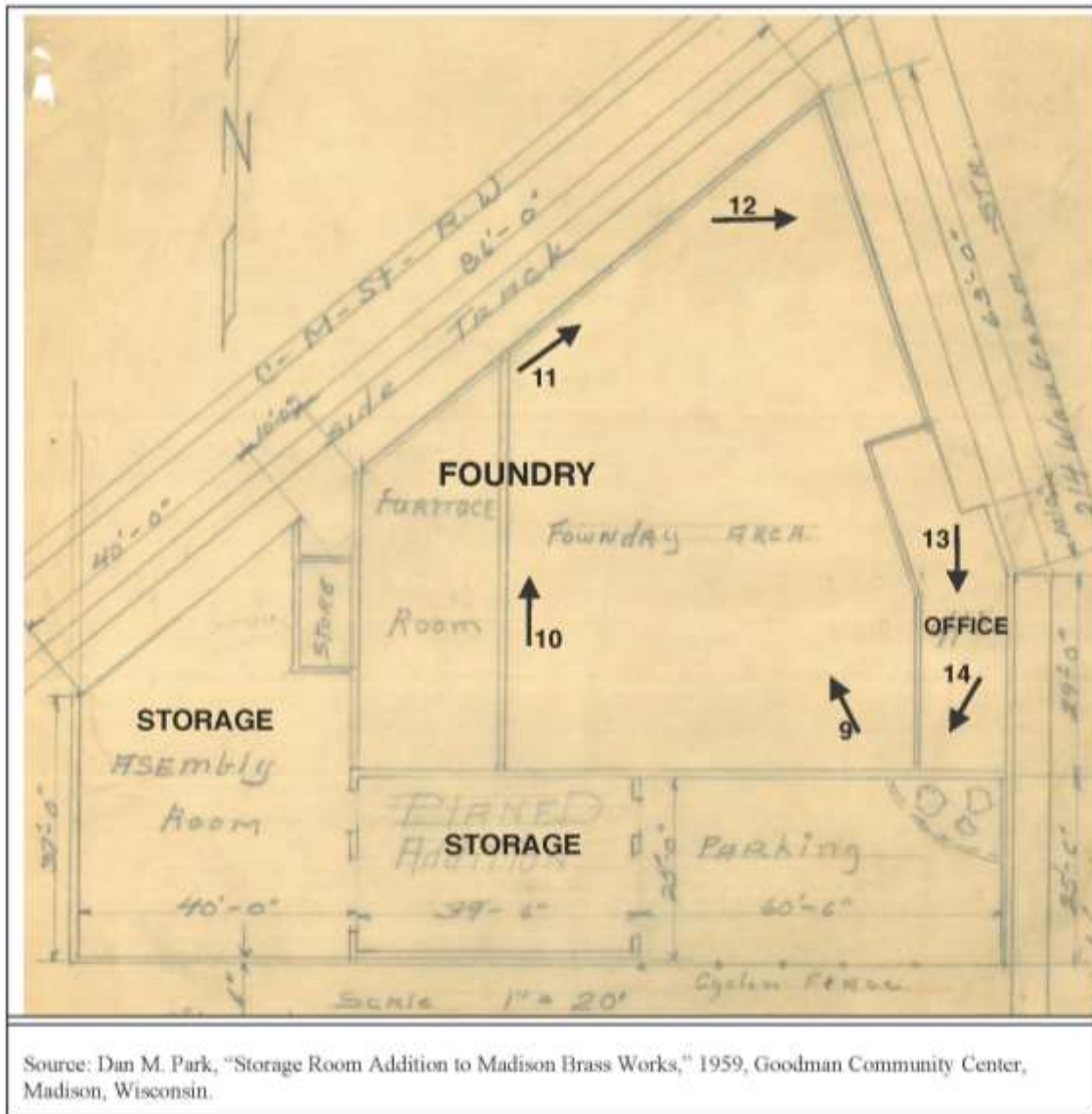
Figure 3. Madison Brass Works, Plan with Photo Key Not to scale
